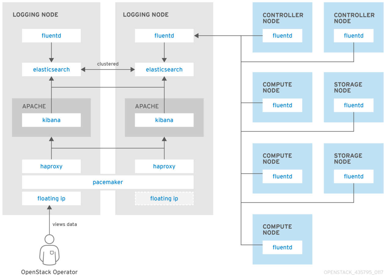
Figure 2.3. HA deployment for Red Hat OpenStack Platform
