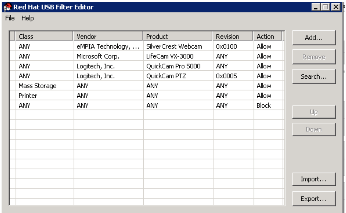
図17.1 Red Hat USB Filter Editor
