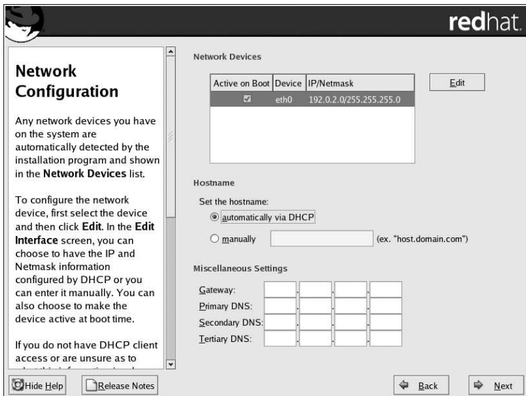
Figure 4-16. Network Configuration
