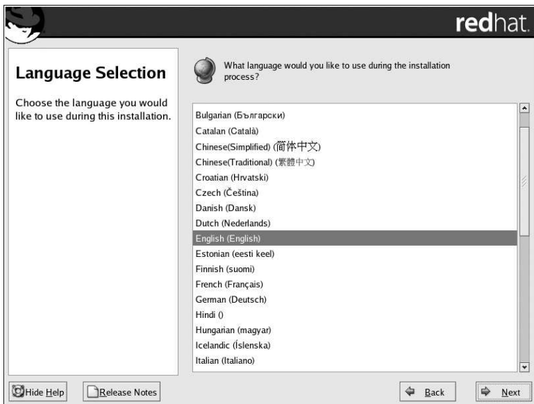
Figure 4-7. Language Selection
