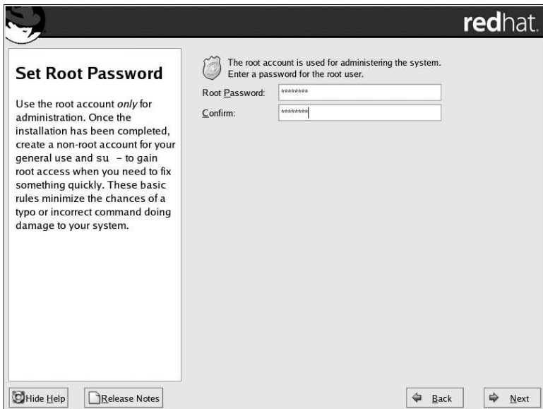
Figure 4-21. Root Password
