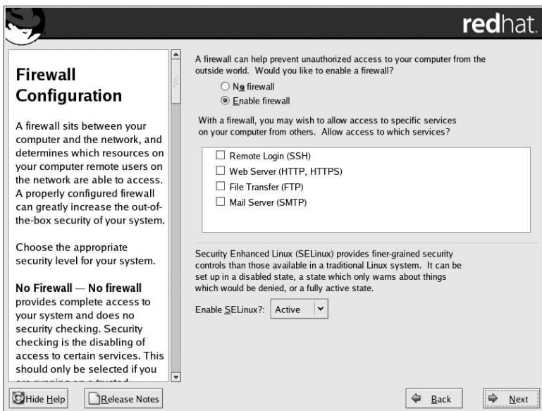
Figure 4-18. Firewall Configuration
