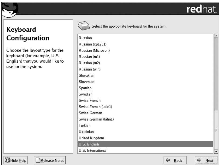
Figure 4-8. Keyboard Configuration
