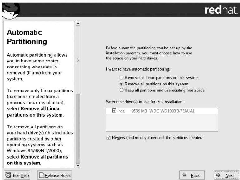
Figure 4-10. Automatic Partitioning
