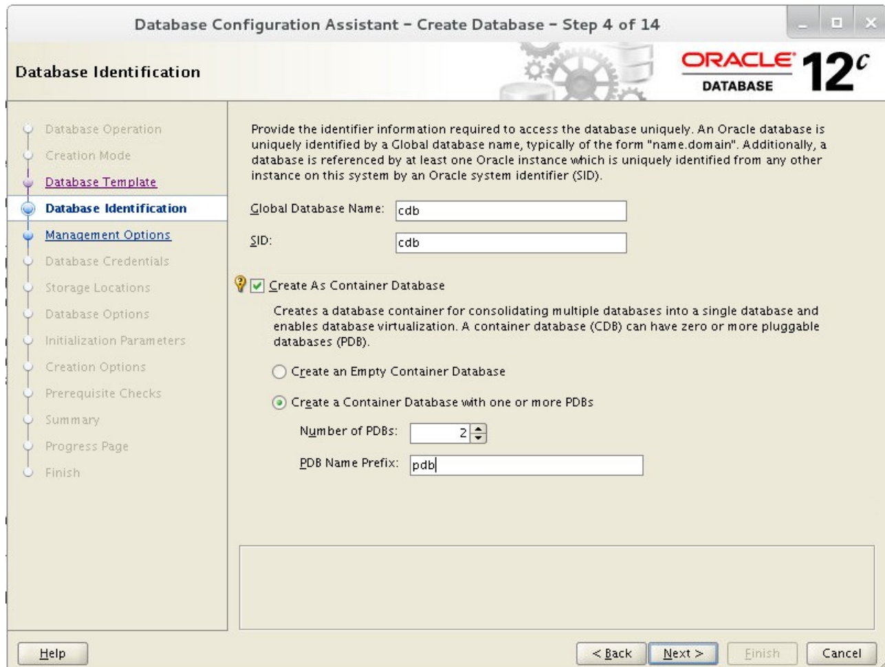
Figure 4.1.4.1: Database Identification Window
