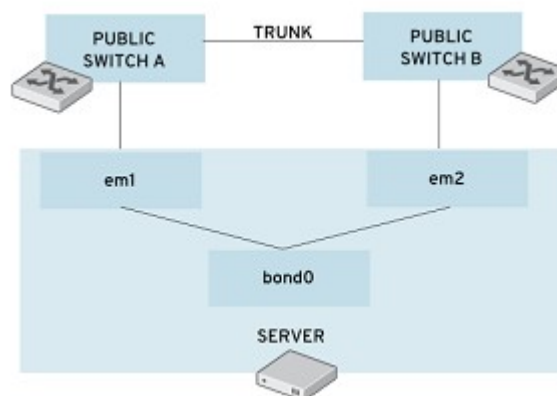
Figure 2.2.2: Ethernet Bonding
