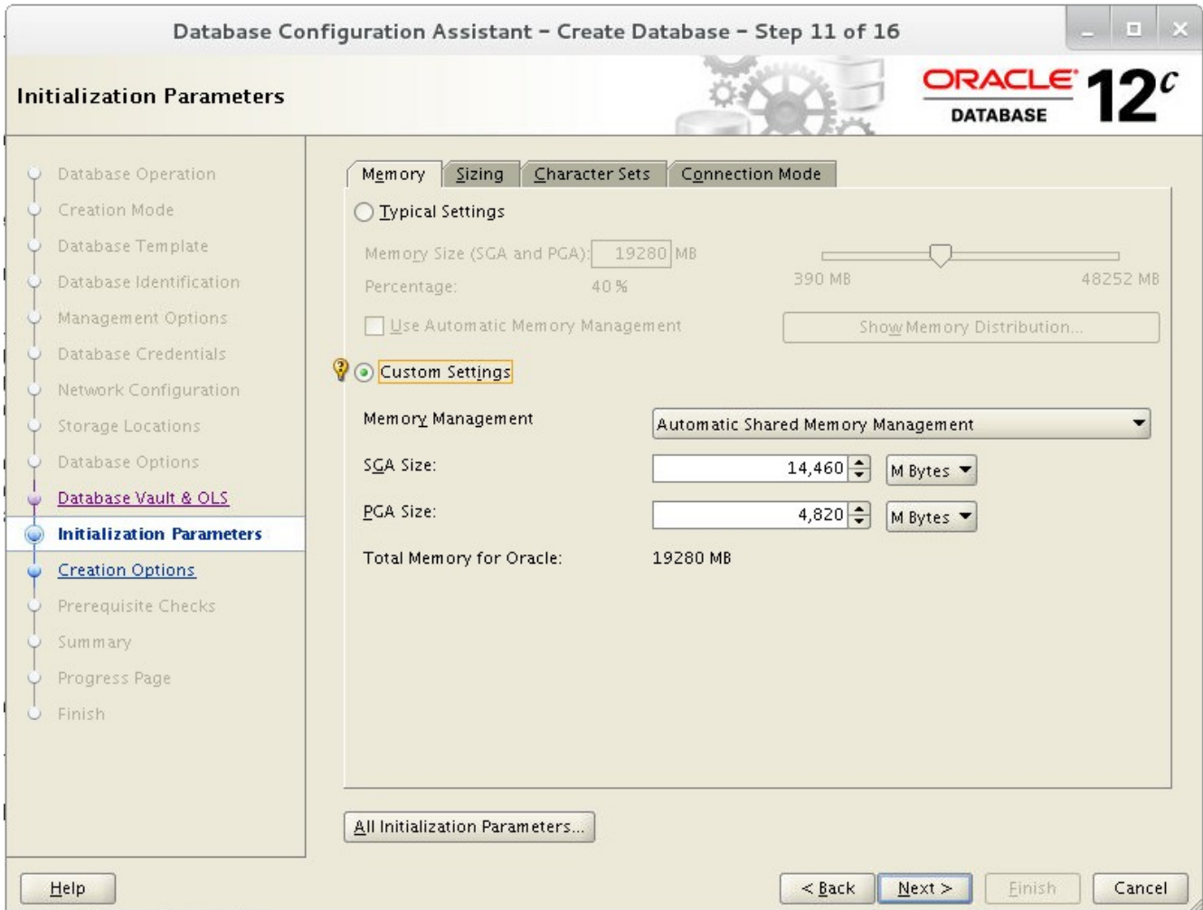
Figure 4.1.4.4: Initialization Parameters Window, Memory Tab
