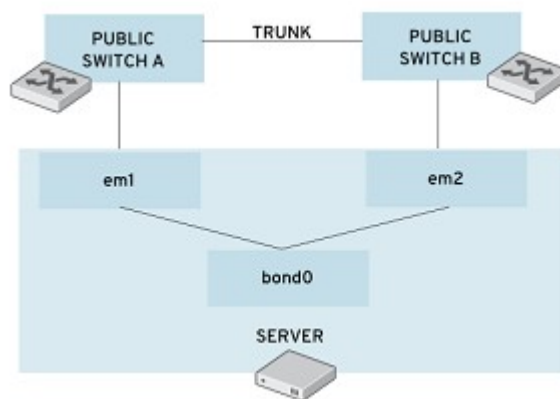
Figure 2.2.2: Ethernet Bonding
