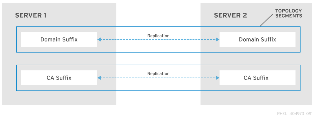
Figure 6.2. Topology Segments
