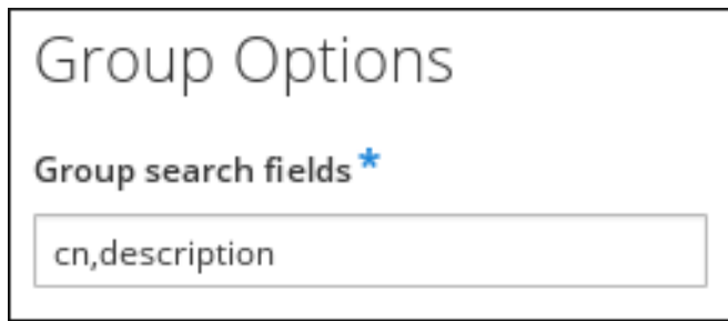
Figure 15.6. Group Attributes
