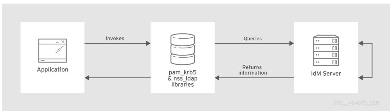
Figure 40.3. Clients and IdM with LDAP and Kerberos
