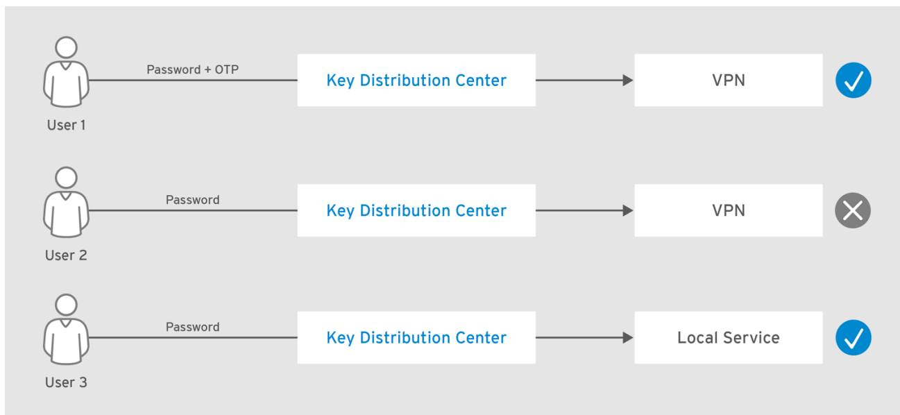
Figure 22.8. Example of Authenticating Using Different Methods
