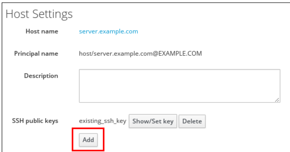
Figure 12.5. Adding an SSH Key
