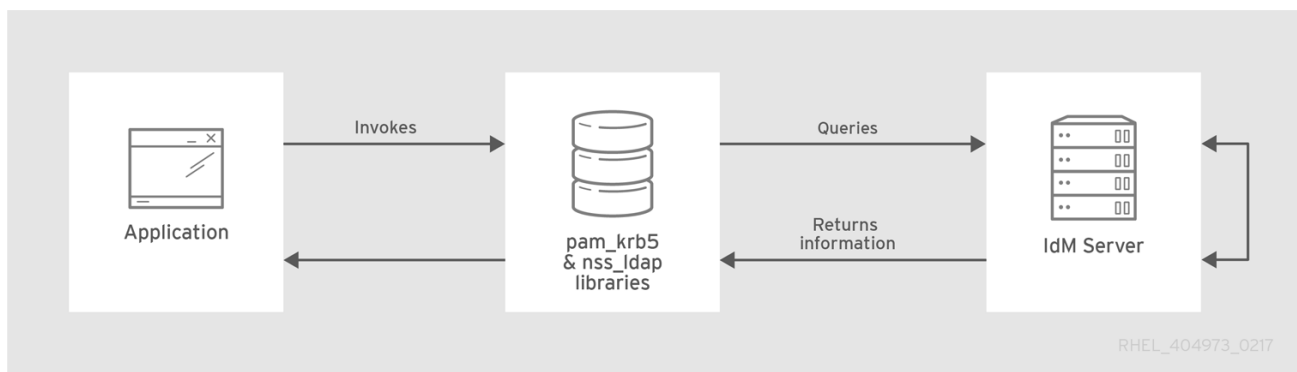
Figure 38.3. Clients and IdM with LDAP and Kerberos
