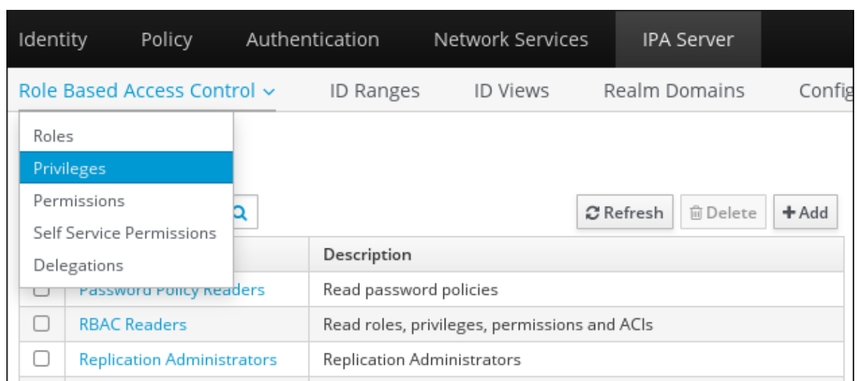
Figure 24.16. Privileges Task
