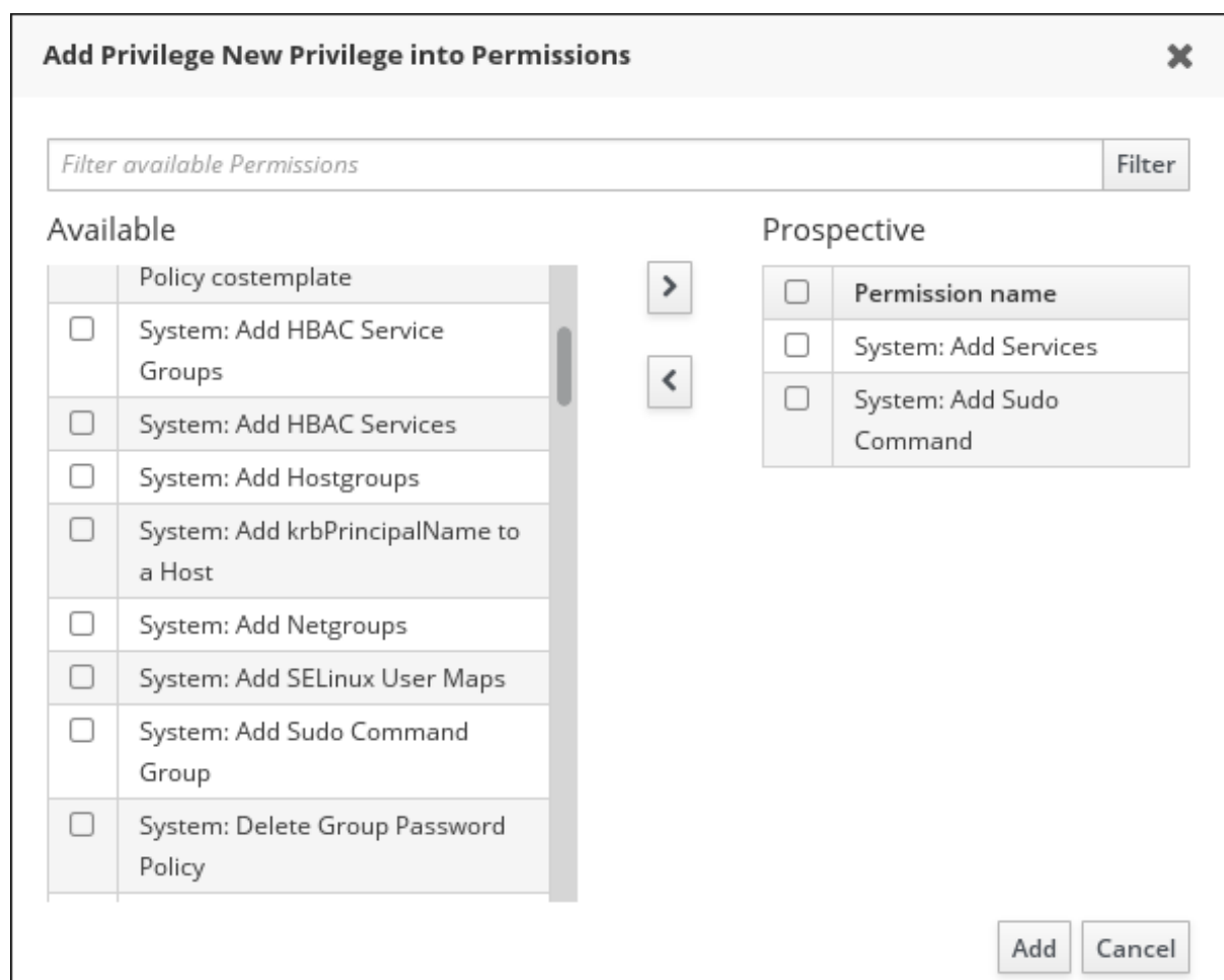
Figure 24.20. Selecting Permissions
