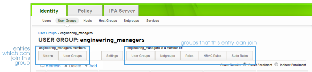
Figure 11.2. Member Of...
