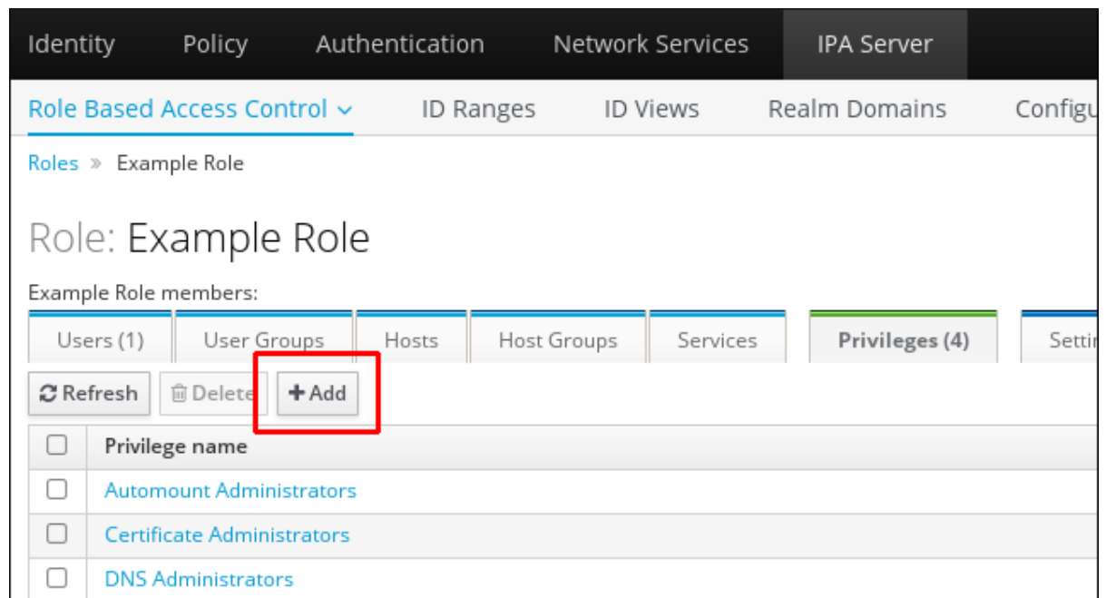
Figure 24.10. Adding Privileges
