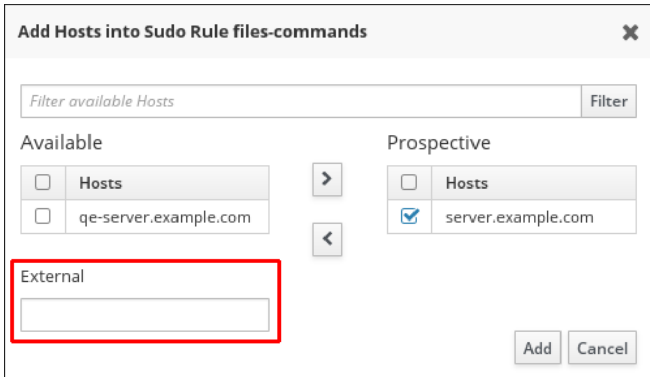
Figure 19.1. External Entities
