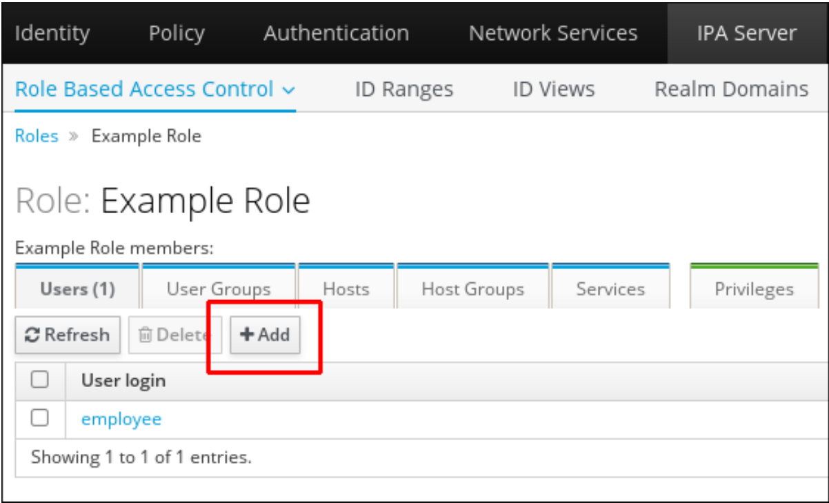
Figure 24.8. Adding Users
