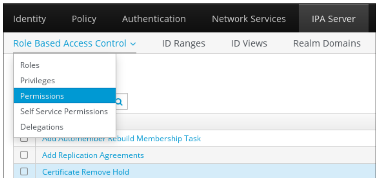
Figure 24.12. Permissions Task
