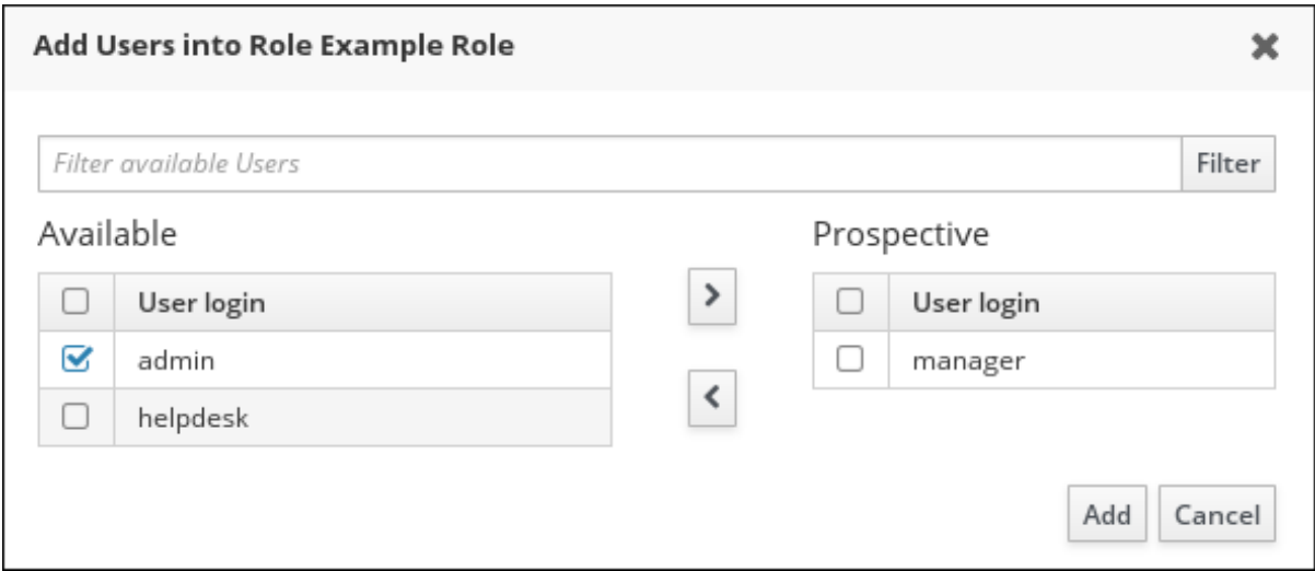
Figure 24.9. Selecting Users
