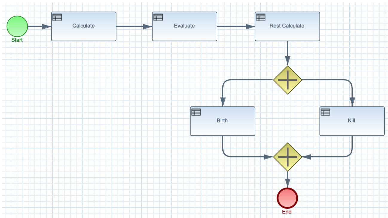
Figure 7.26. Generation ruleflow
