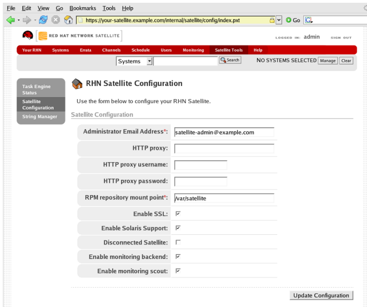
Figure 8.2. Enabling UNIX Support After Satellite Installation
