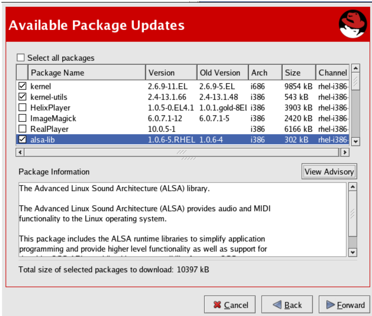
Figure 2.11. Available Package Updates
