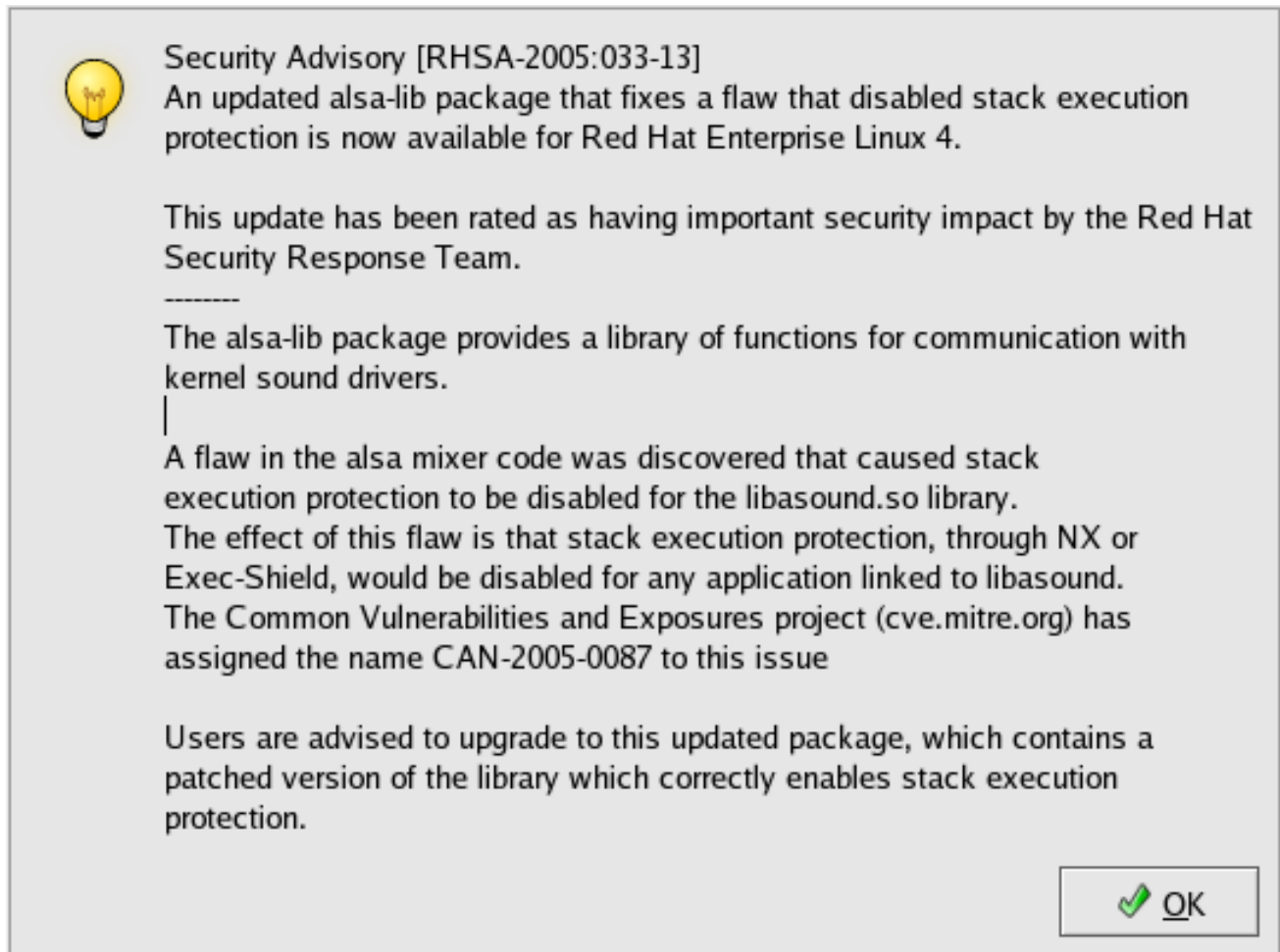
Figure 2.12. Example Errata Advisory
