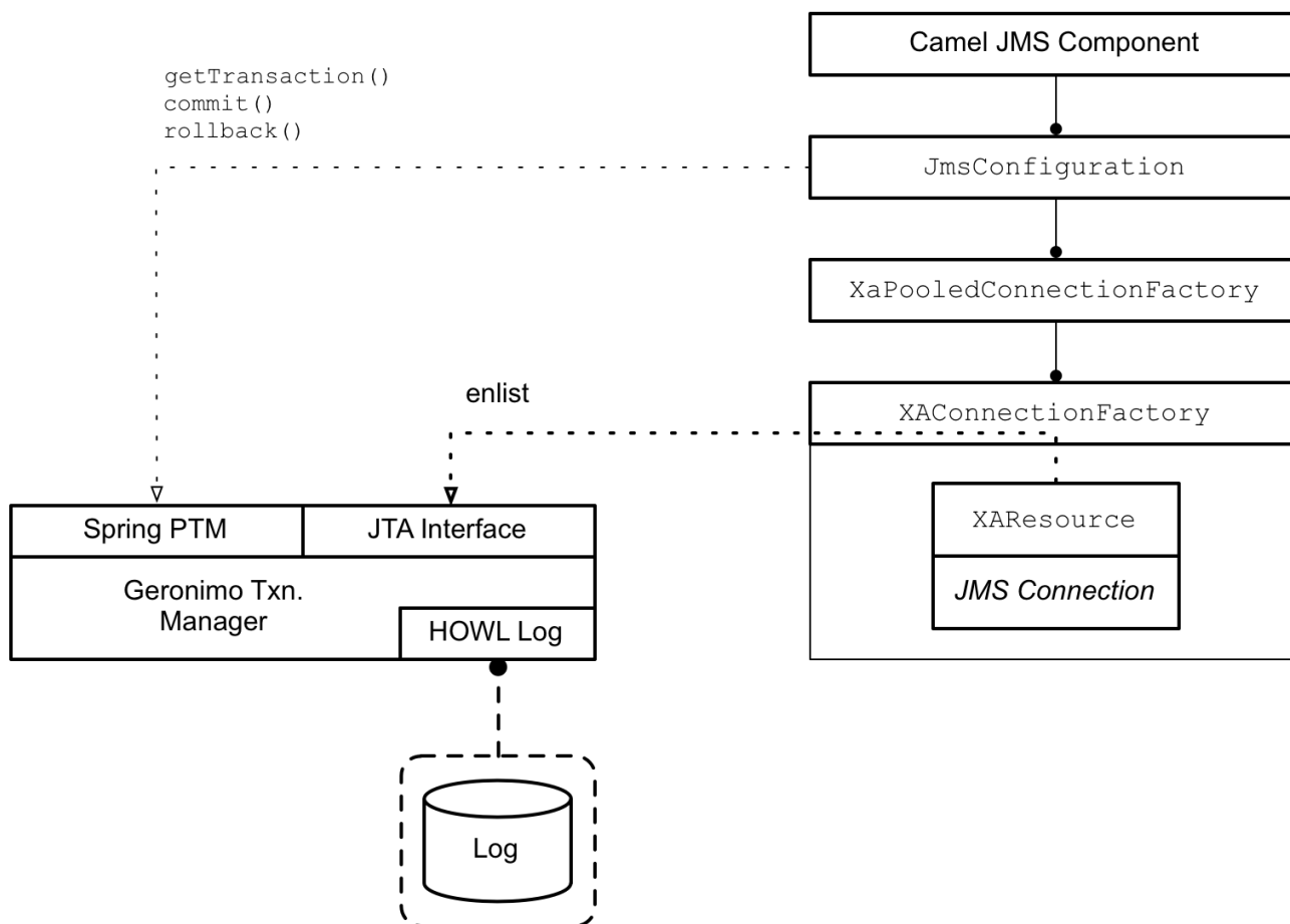
Figure 7.1. Camel JMS Component Integrated with XA Transactions
