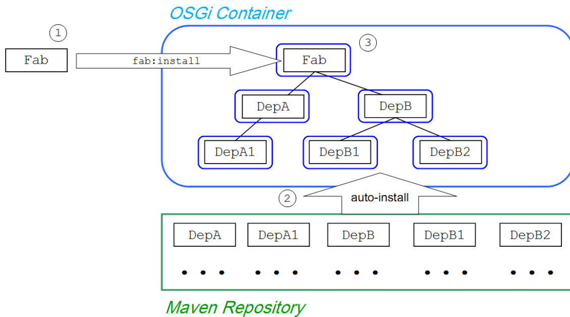
Figure 12.2. FAB Installed with Shared Dependencies
