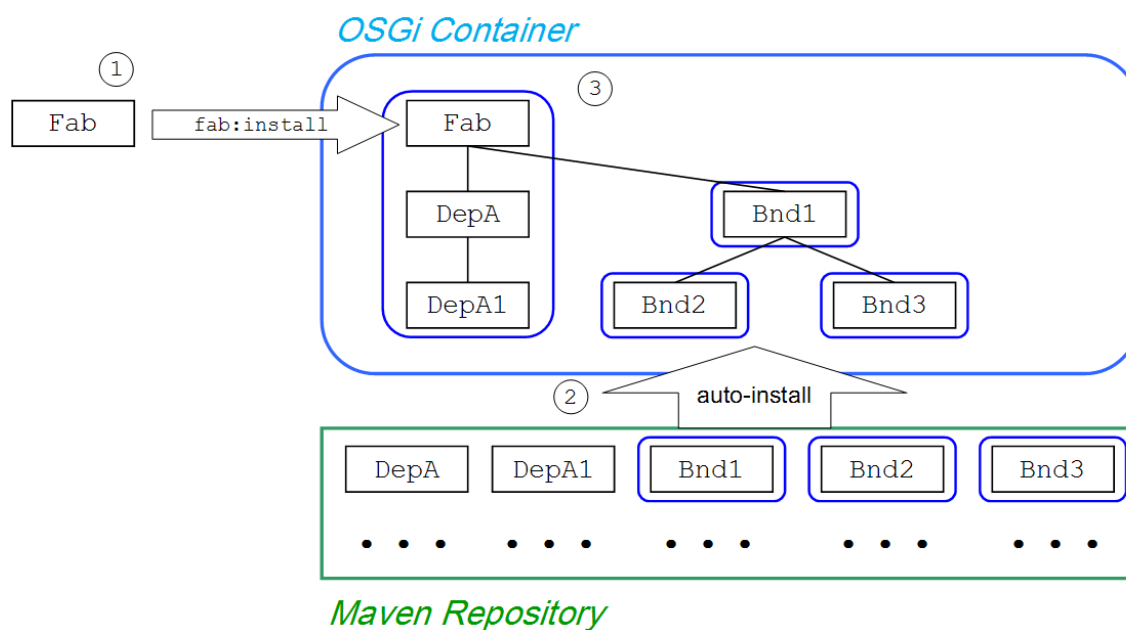
Figure 12.4. Default FAB Install Behavior
