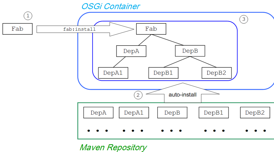
Figure 12.1. FAB Installed with Private Dependencies
