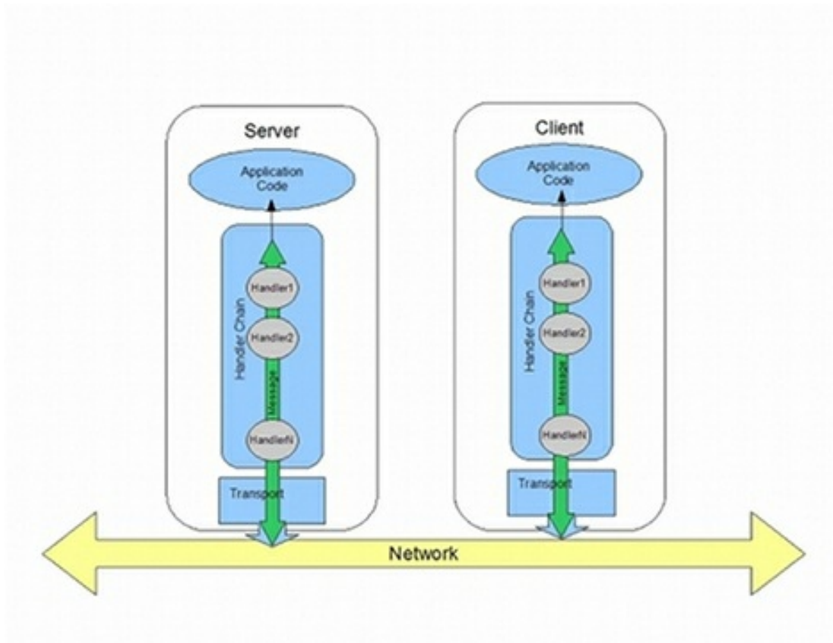
Figure 21.2. Message Exchange Path with Handlers
