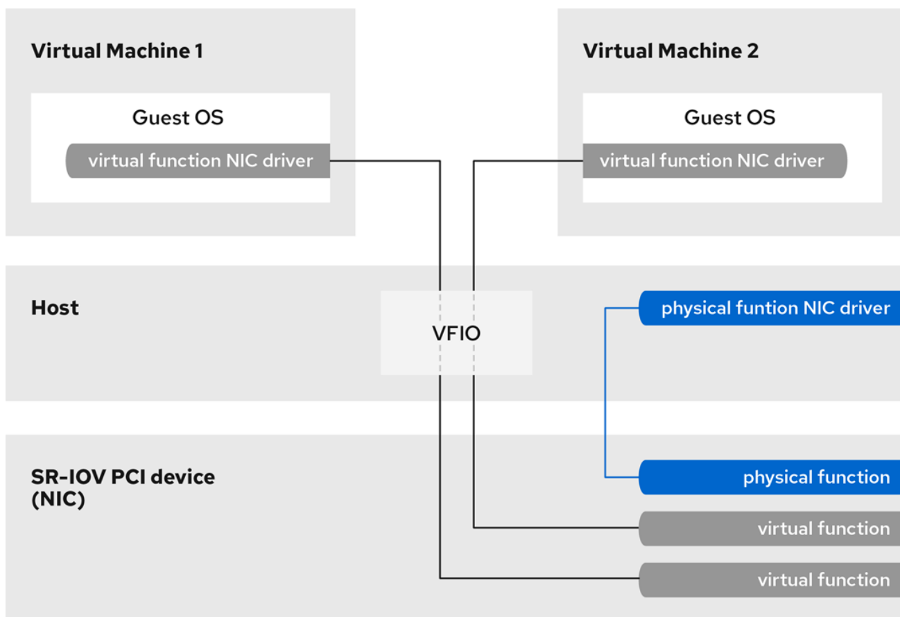
Figure 14.1. SR-IOV architecture
