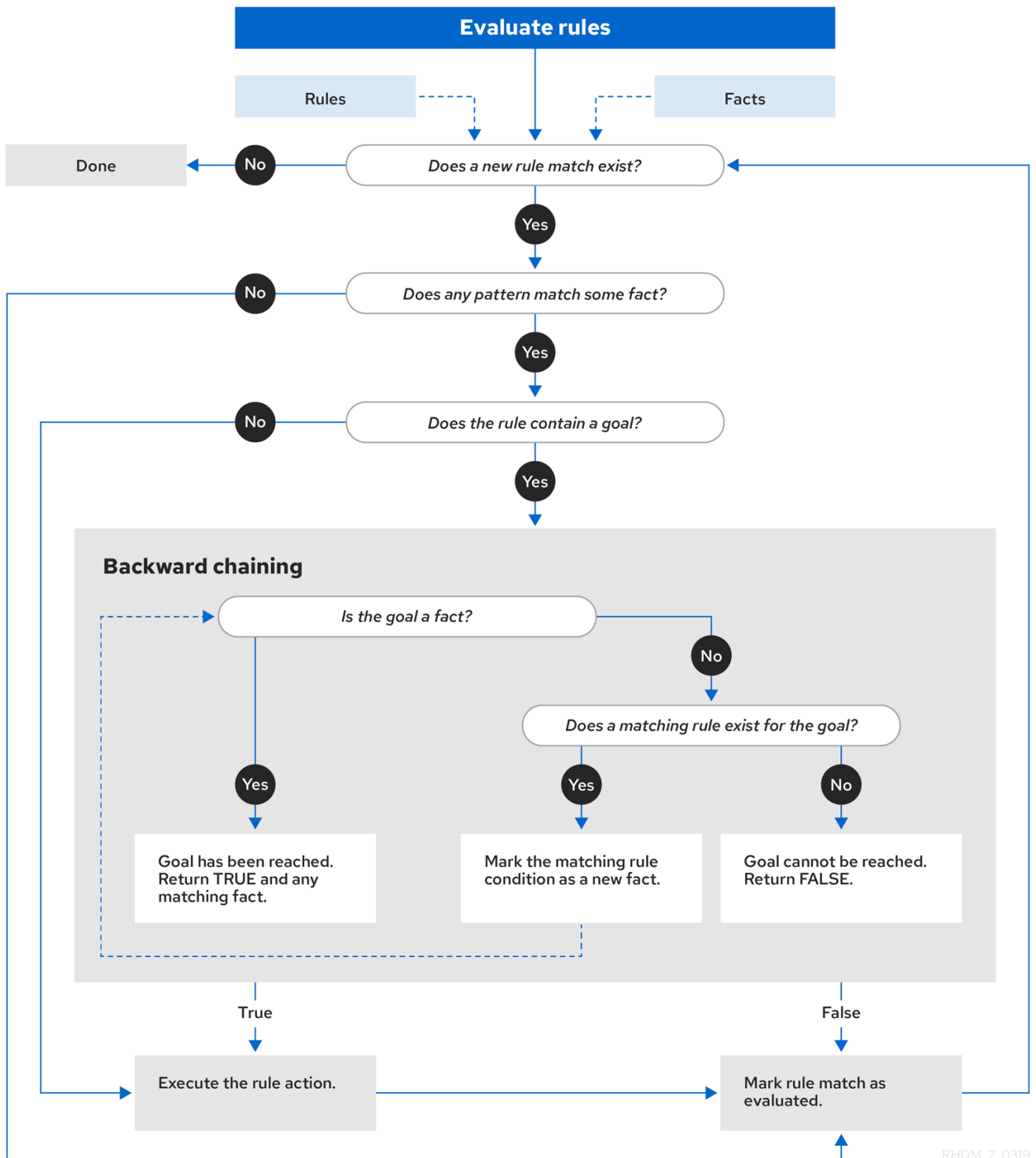
Figure 84.7. Rule evaluation logic using forward and backward chaining
