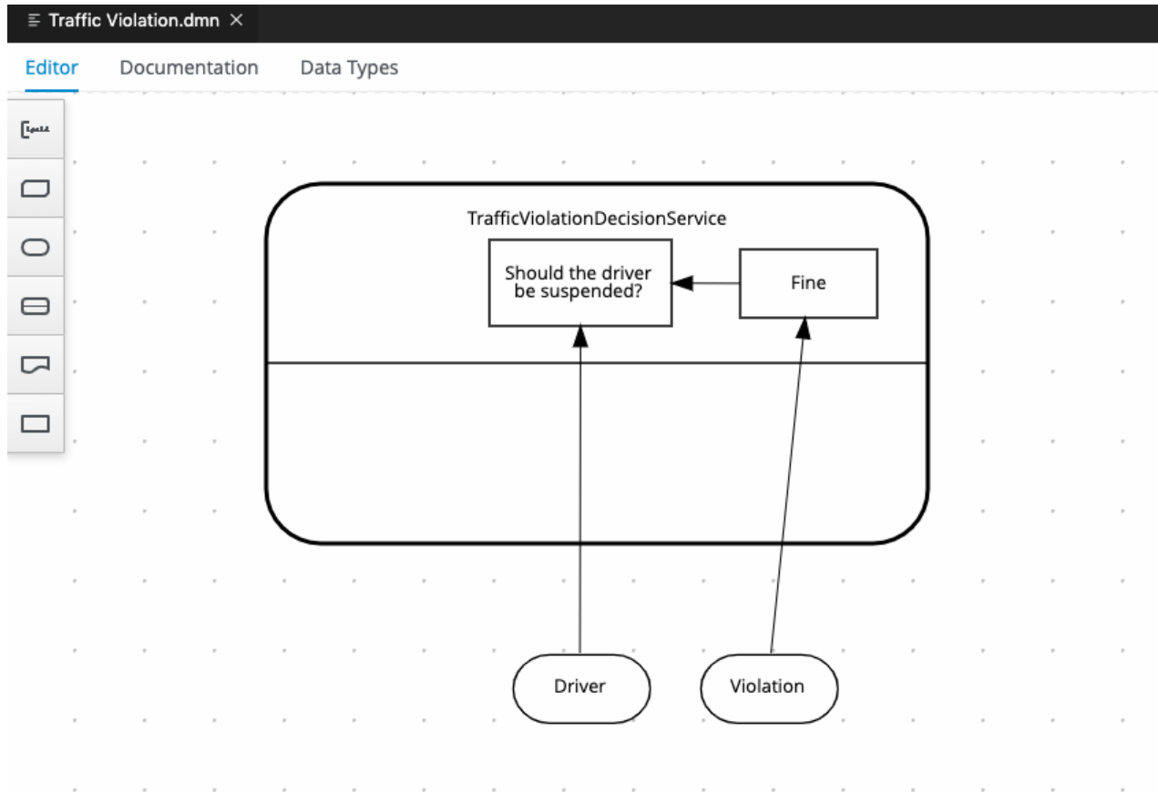
Figure 7.2. Example TrafficViolationDecisionService decision service with multiple-output decision
