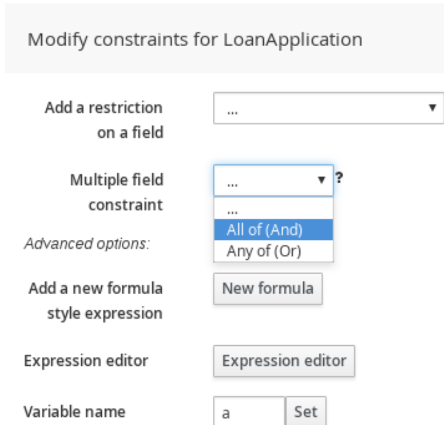
Figure 52.4. Add multiple field constraints
