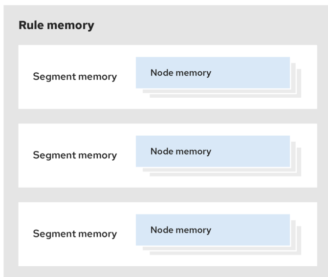
Figure 84.1. Phreak three-layered memory system
