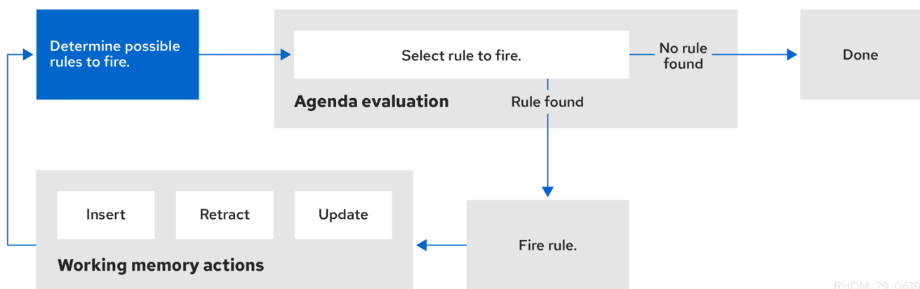
Figure 83.1. Two-phase execution process in the decision engine
