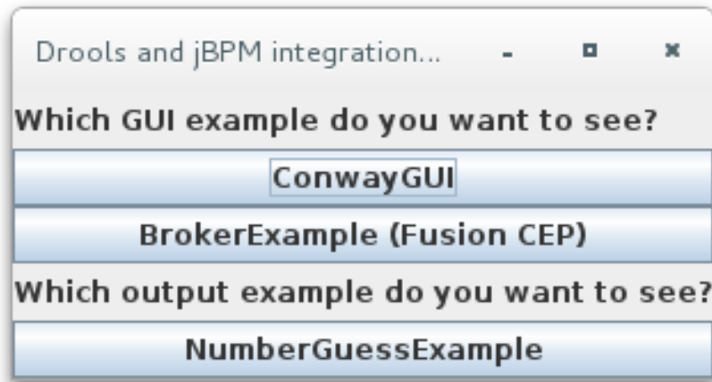
Figure 89.2. Interface for all examples in droolsjbpm-integration-examples (DroolsJbpmIntegrationExamplesApp.java)
