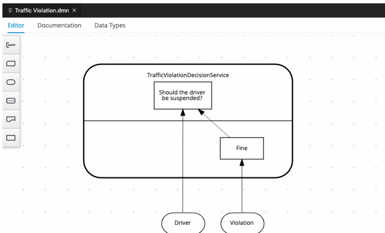
Figure 7.1. Example TrafficViolationDecisionService decision service with single-output decision
