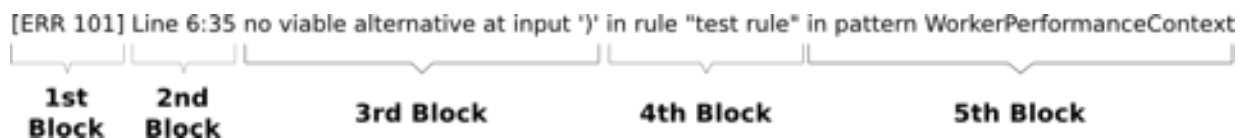
Figure 16.1. Error message format for DRL file problems
