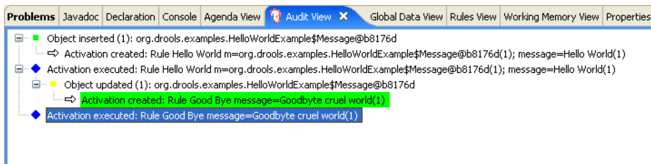
Figure 89.3. Hello World example Audit View
