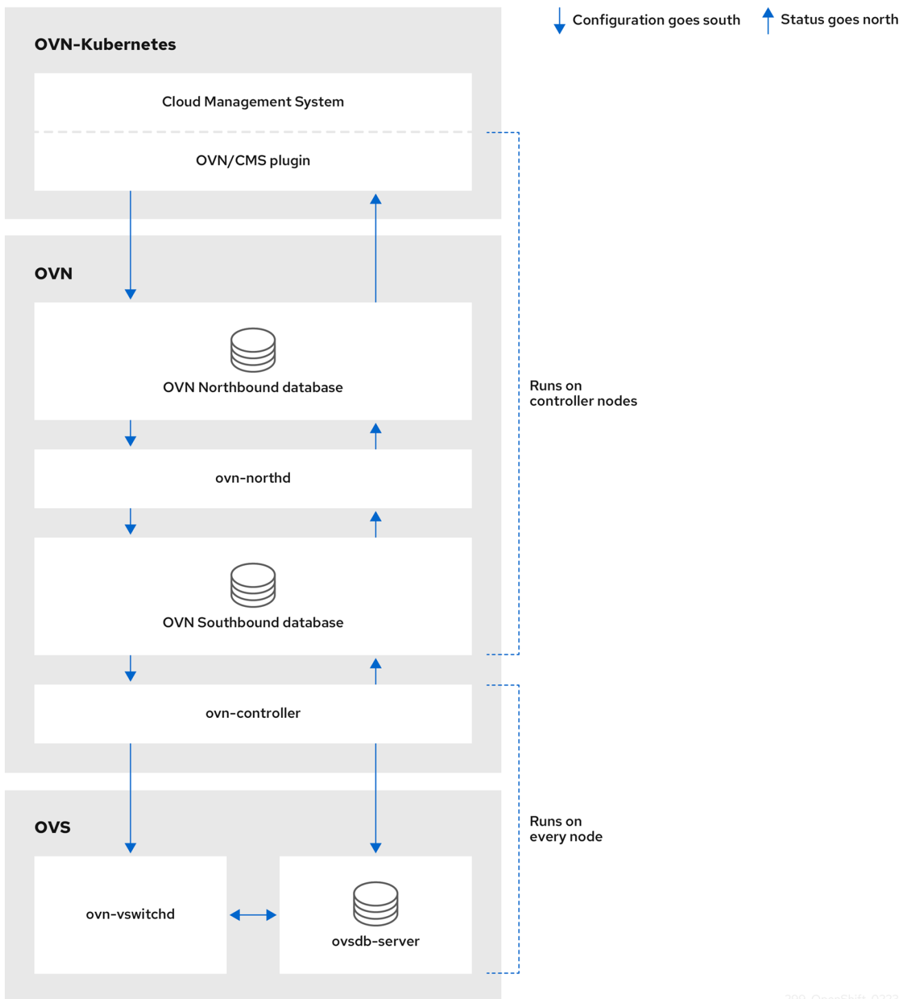
Figure 25.1. OVK-Kubernetes architecture
