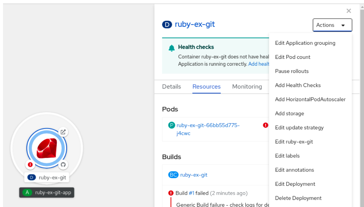
Figure 2.2. Add HorizontalPodAutoscaler
