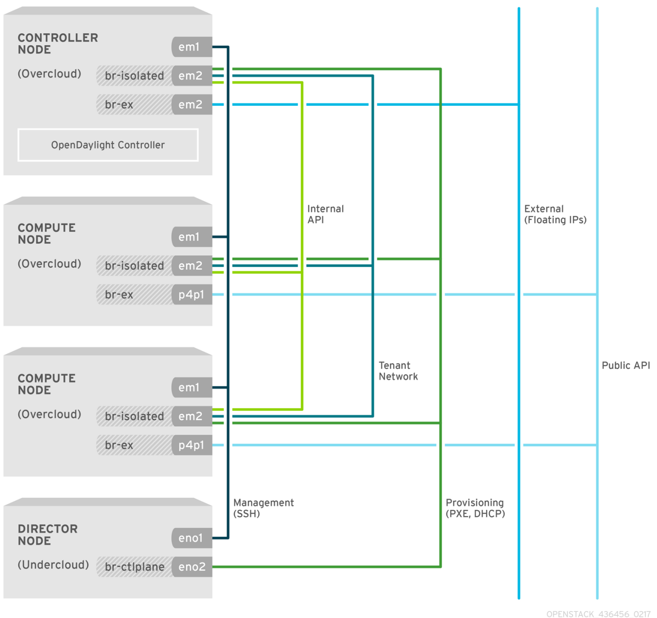
Figure 7.1. Detailed network topology used in this scenario
