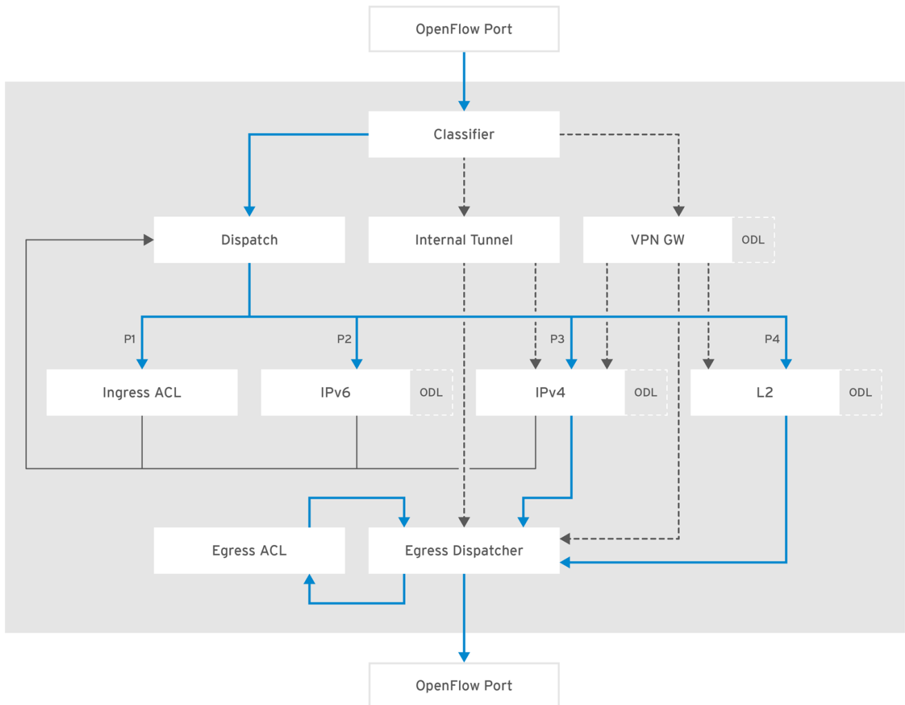
Figure 6.1. OpenDaylight NetVirt OpenFlow Pipeline
