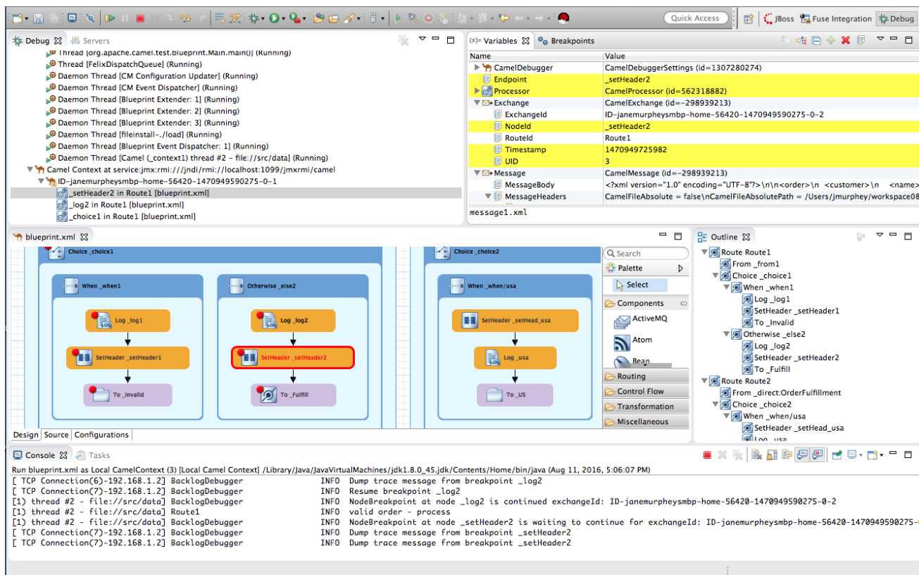
Figure 3.1. Debug perspective
