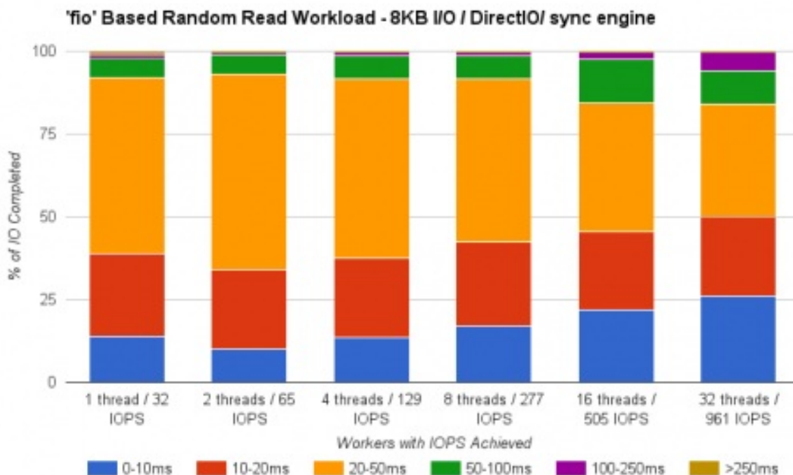
Figure 3.3. Disk Latencies
