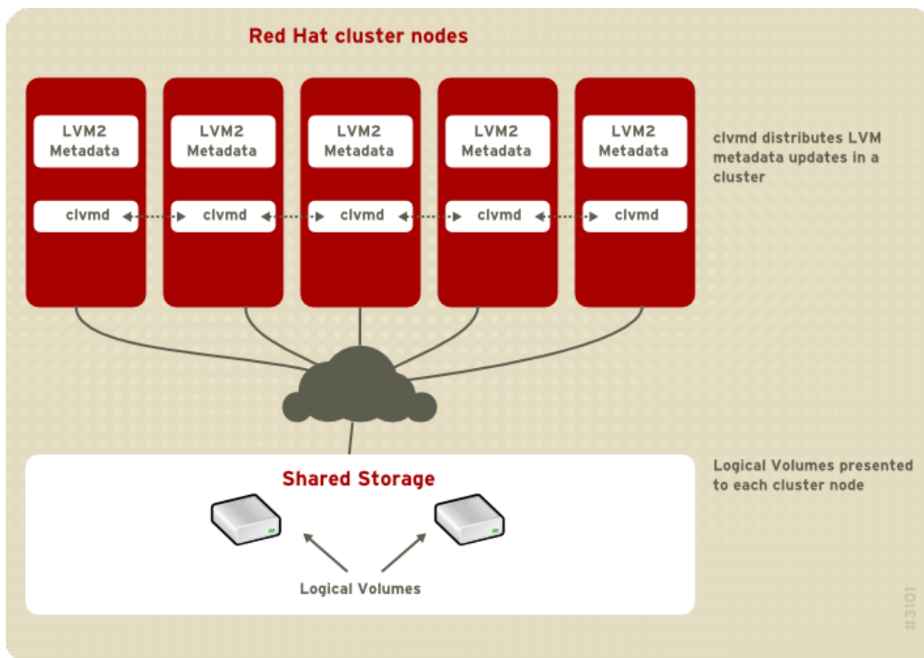
Figure 2.2. CLVM Overview
