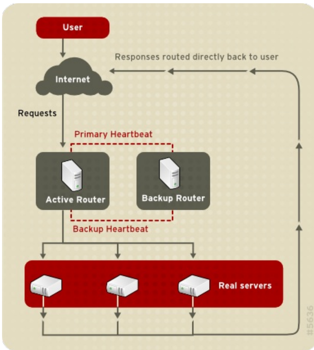
Figure 1.4. Load Balancer Add-On Implemented with Direct Routing
