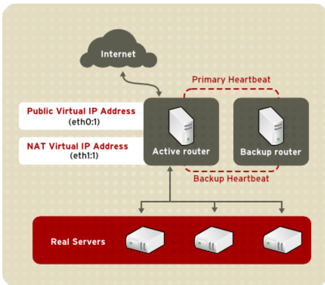
Figure 1.3. Load Balancer Add-On Implemented with NAT Routing
