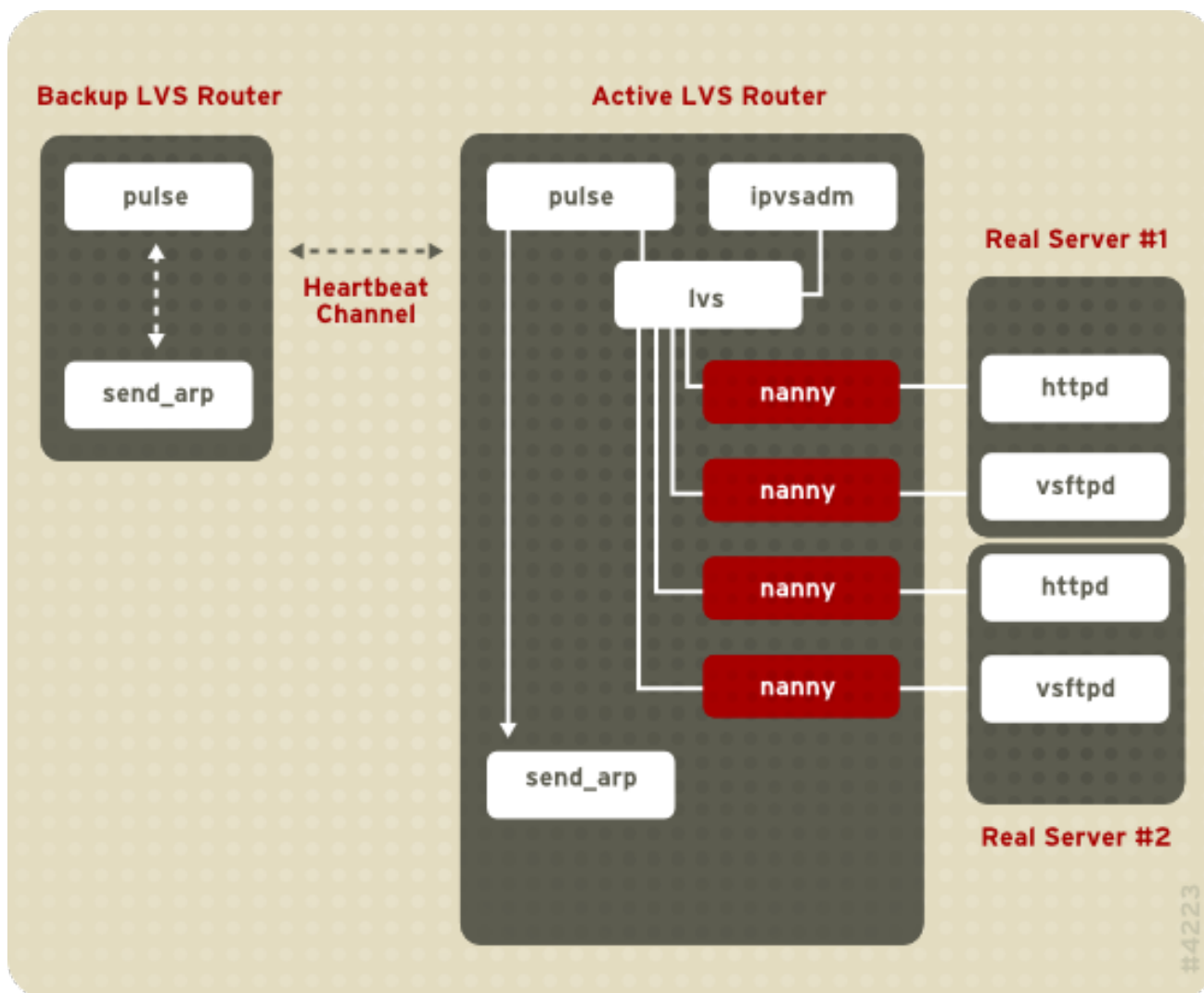
Figure 1.5. Load Balancer Add-On Components
