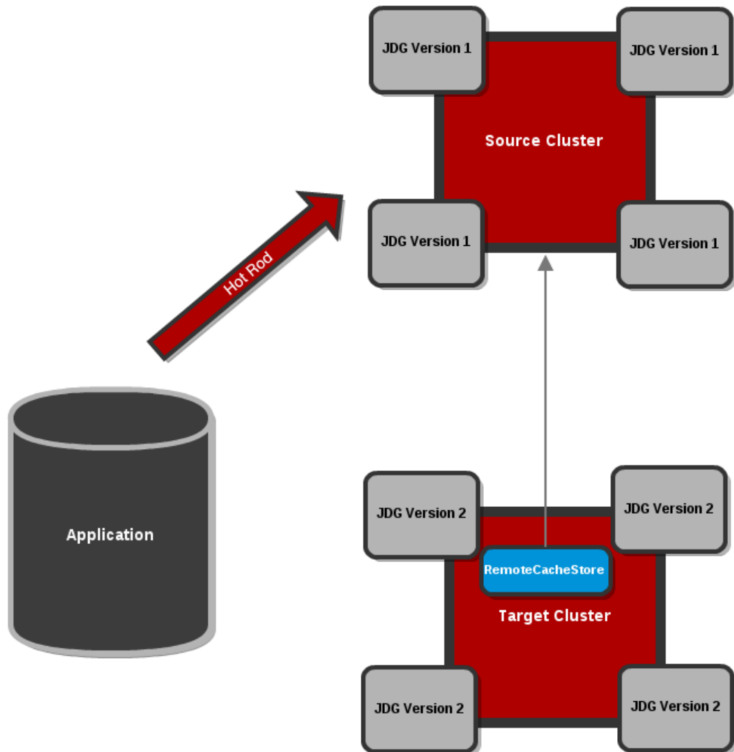
Figure 15.1. Configure the Target Cluster with a RemoteCacheStore
