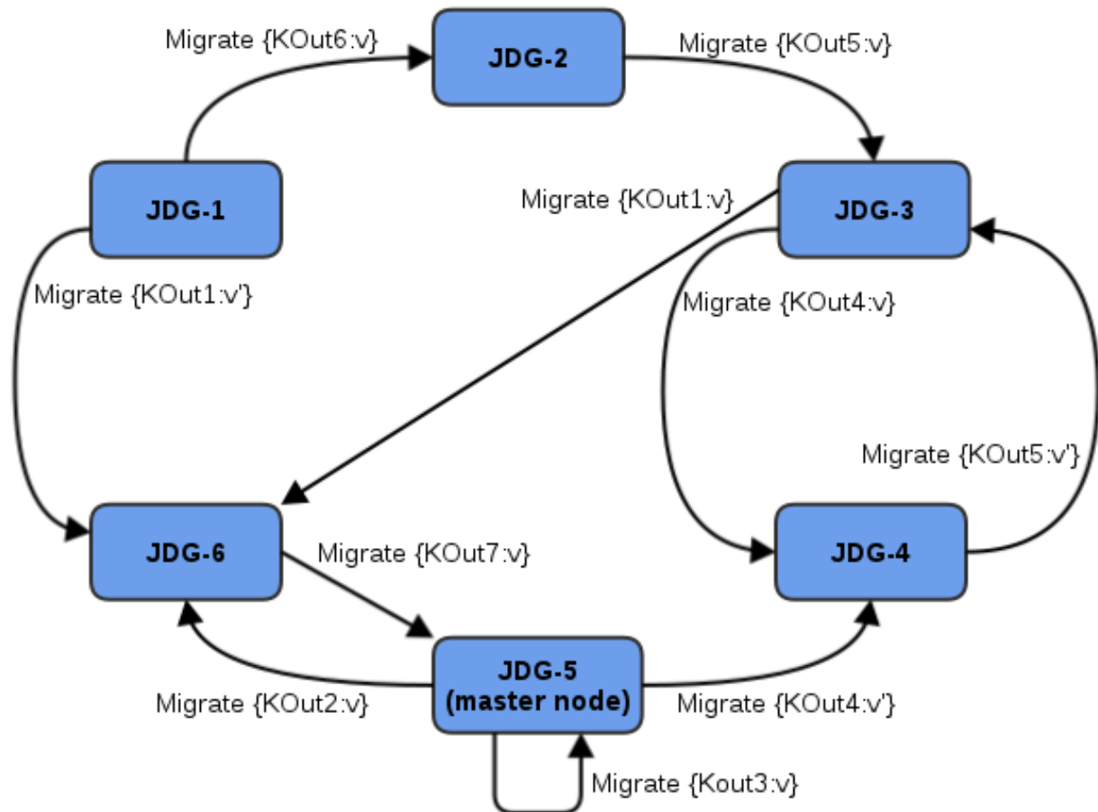
Figure 16.2. Kout/VOut Migration
