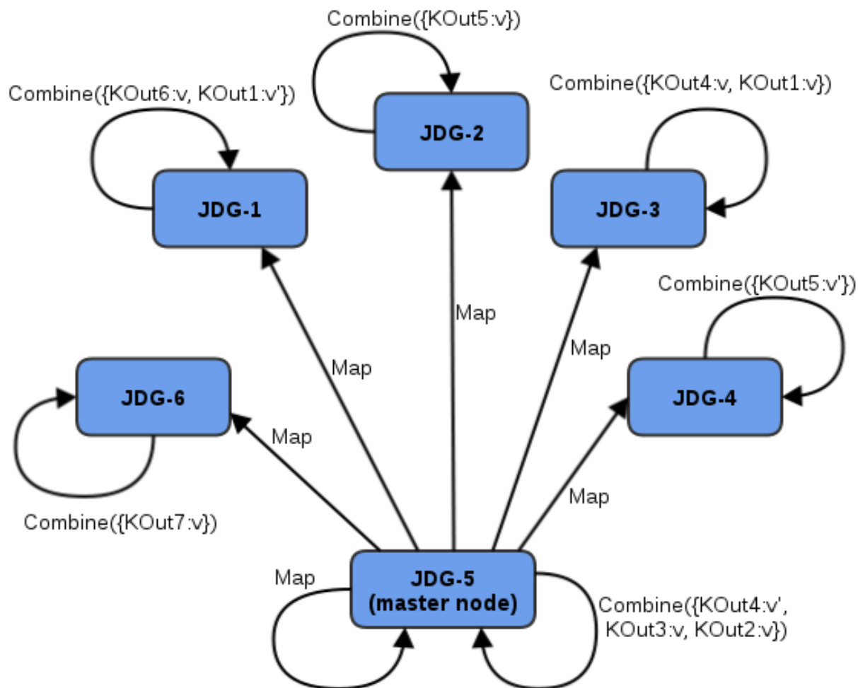
Figure 16.1. Map Phase
