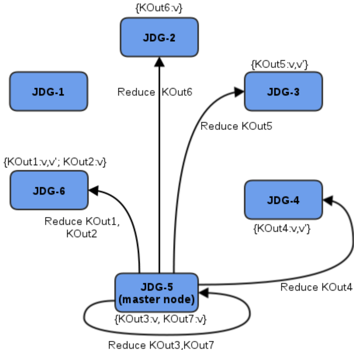
Figure 16.3. Reduce Phase
