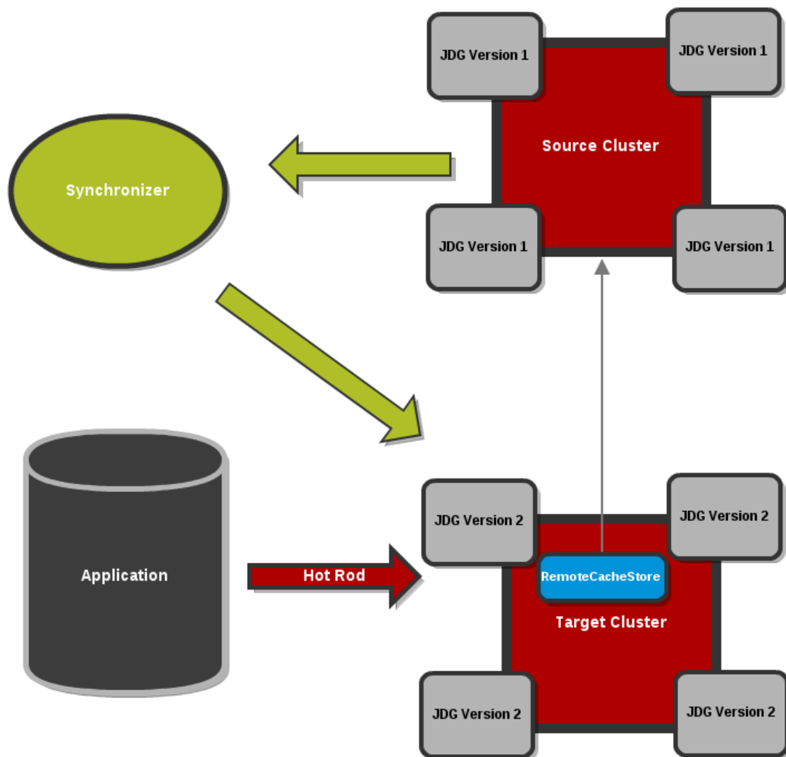
Figure 15.2. Clients point to the Target Cluster with the Source Cluster as RemoteCacheStore for the Target Cluster.
