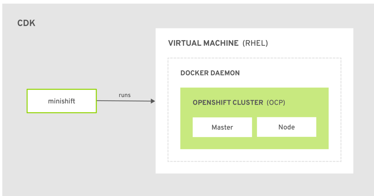
Figure 2.1 : CDK architecture
