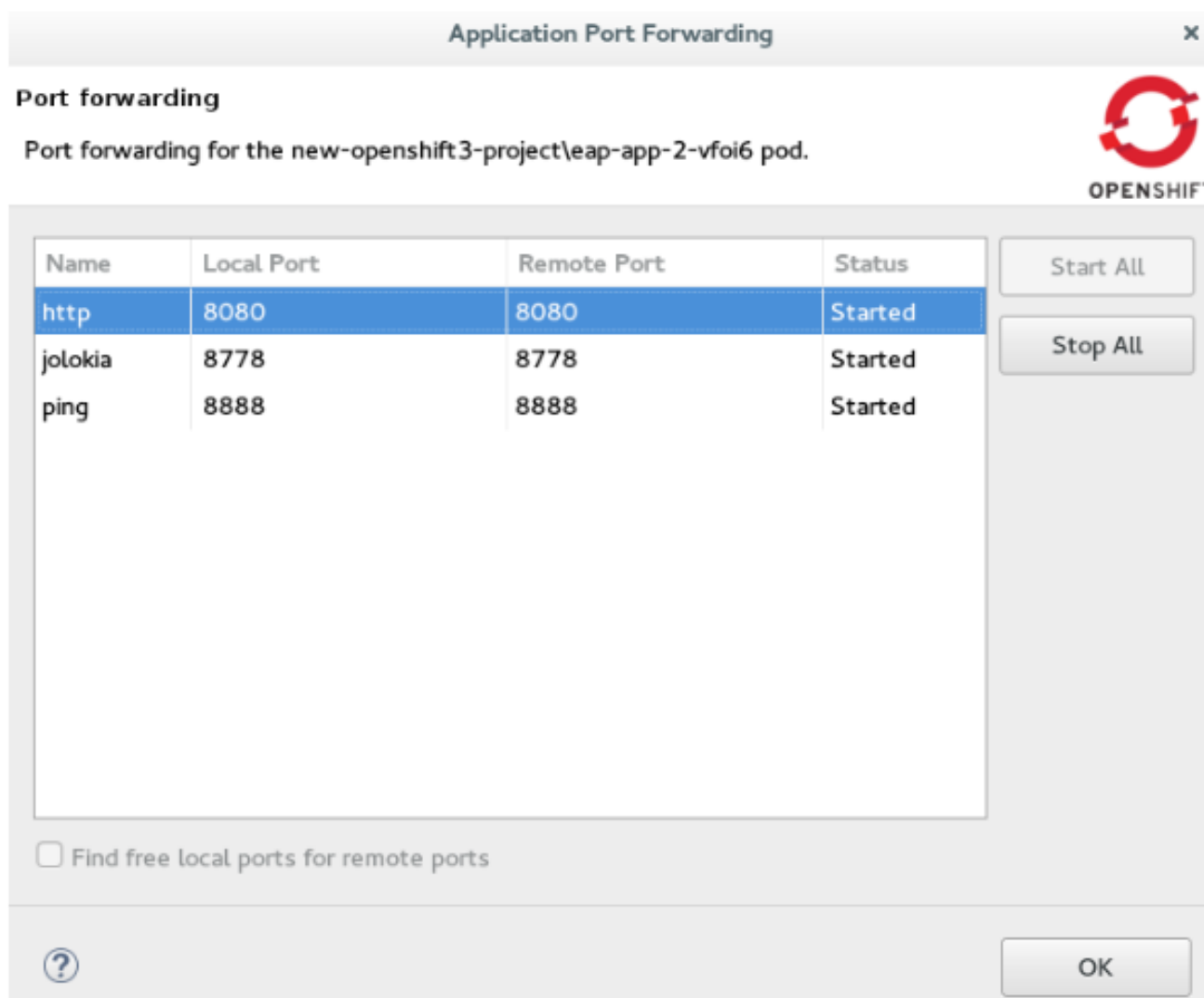
Figure 2.8. Start Port Forwarding
