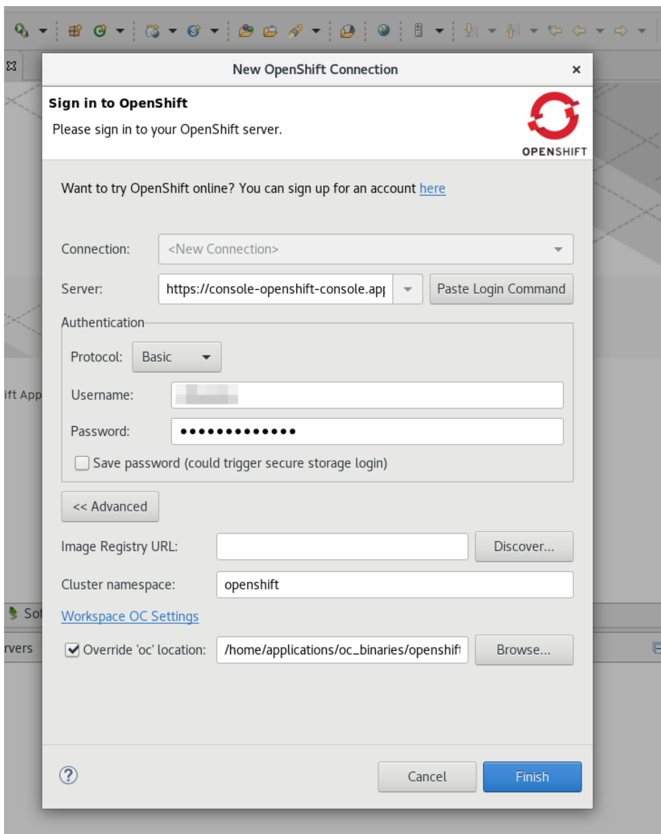
Figure 2.3. Set up a new OpenShift Container Platform connection
