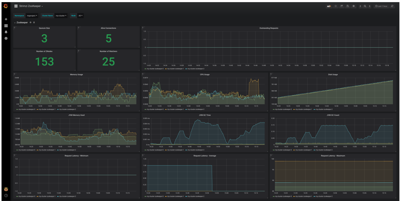
Figure 9.2. Zookeeper dashboard
