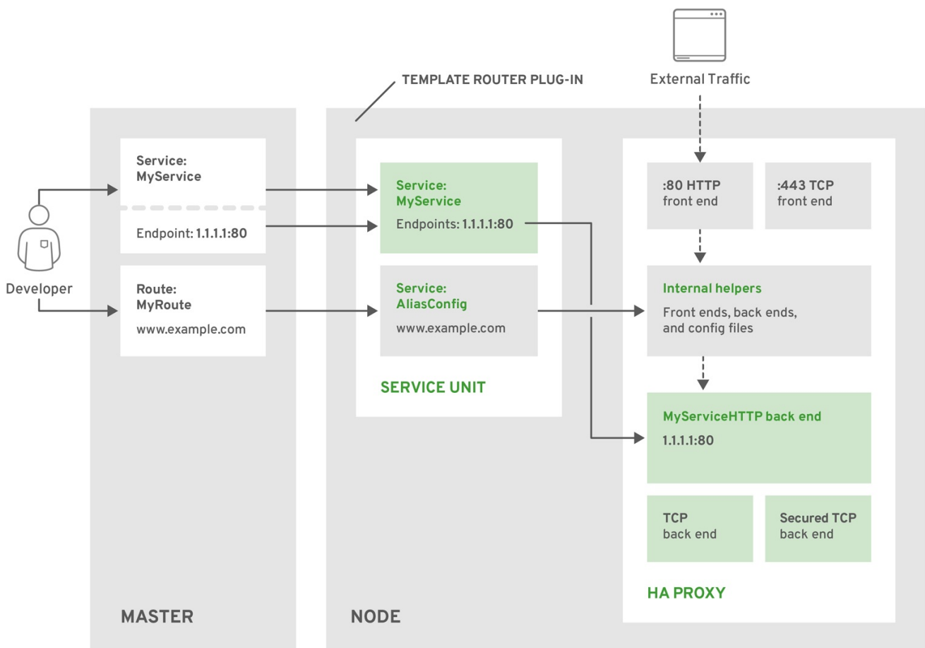
Figure 5.5. HAProxy Router Data Flow
