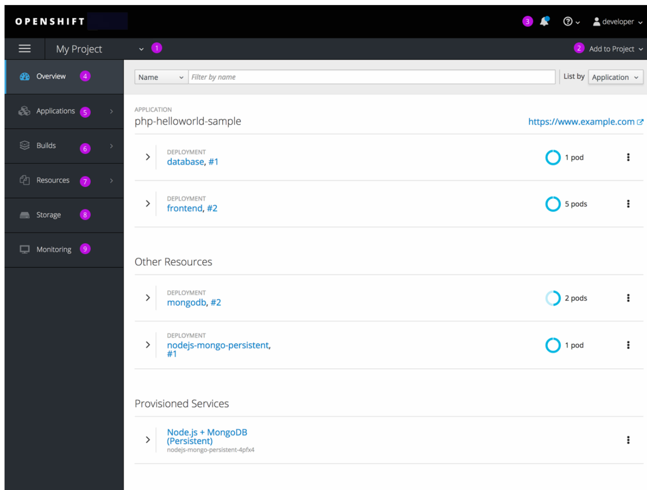
Figure 2.2. Web Console Project Overview
