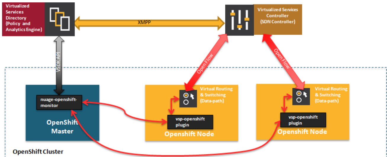
Figure 5.1. Nuage VSP Integration with OpenShift Container Platform
