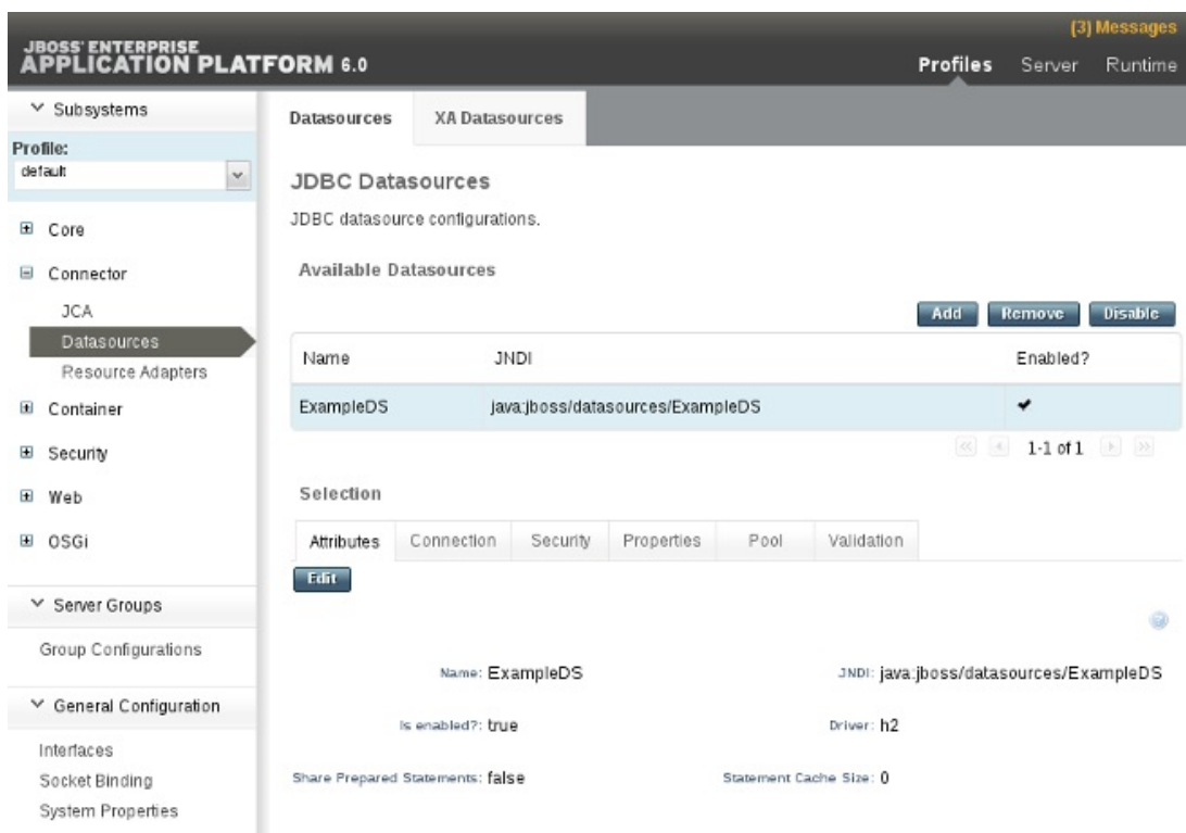
Figure 10.2. Datasources panel
