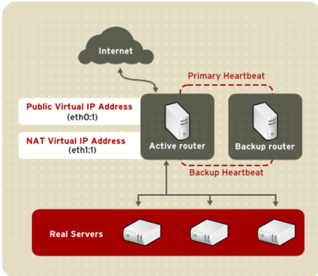
圖形 1.3. LVS Implemented with NAT Routing
