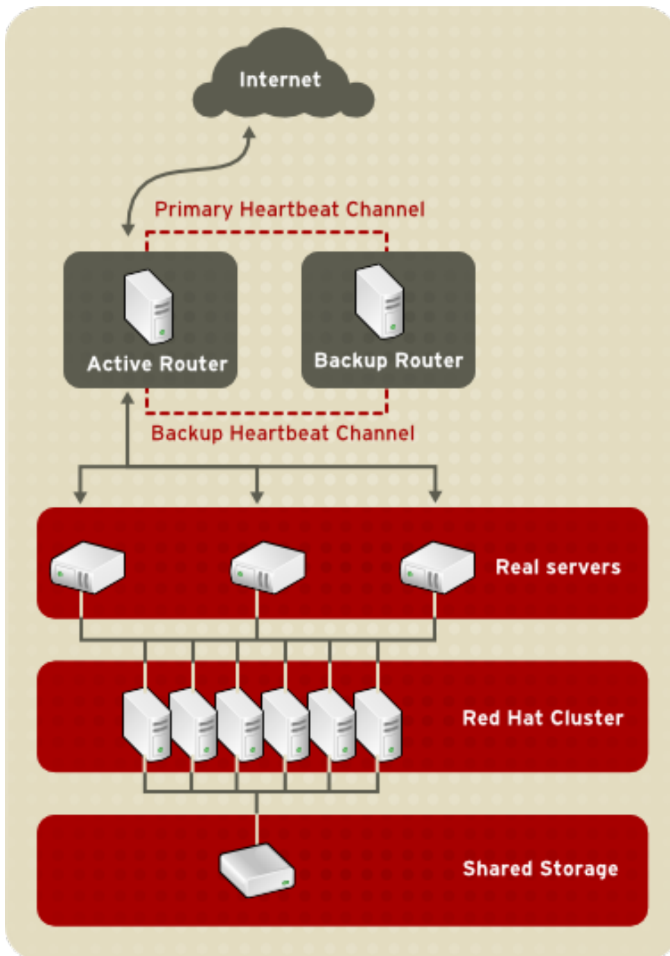
圖形 1.2. A Three-Tier LVS Configuration
