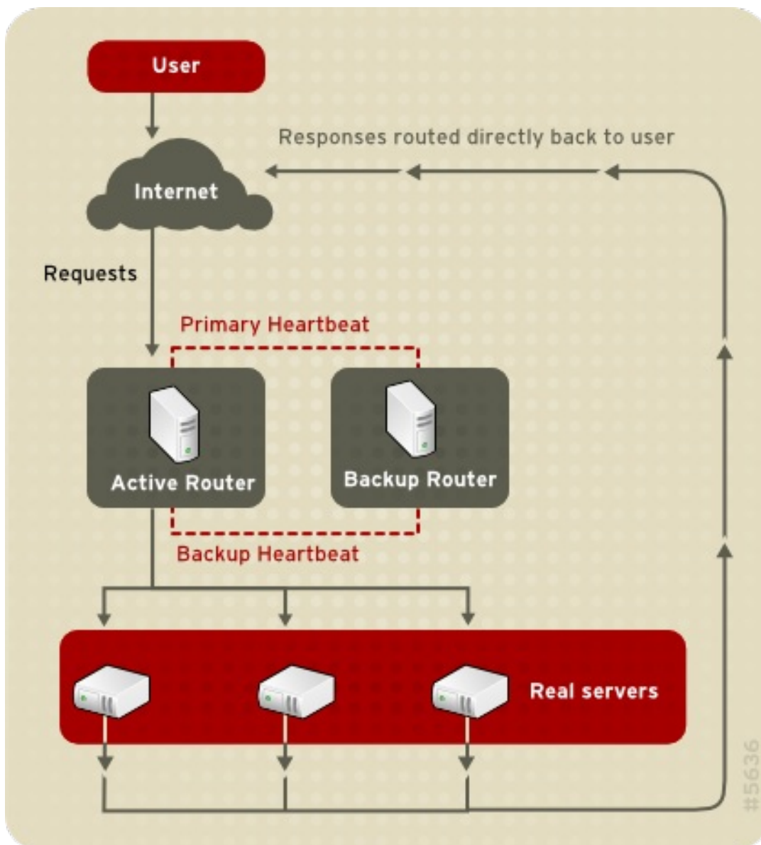
圖形 1.4. LVS Implemented with Direct Routing
