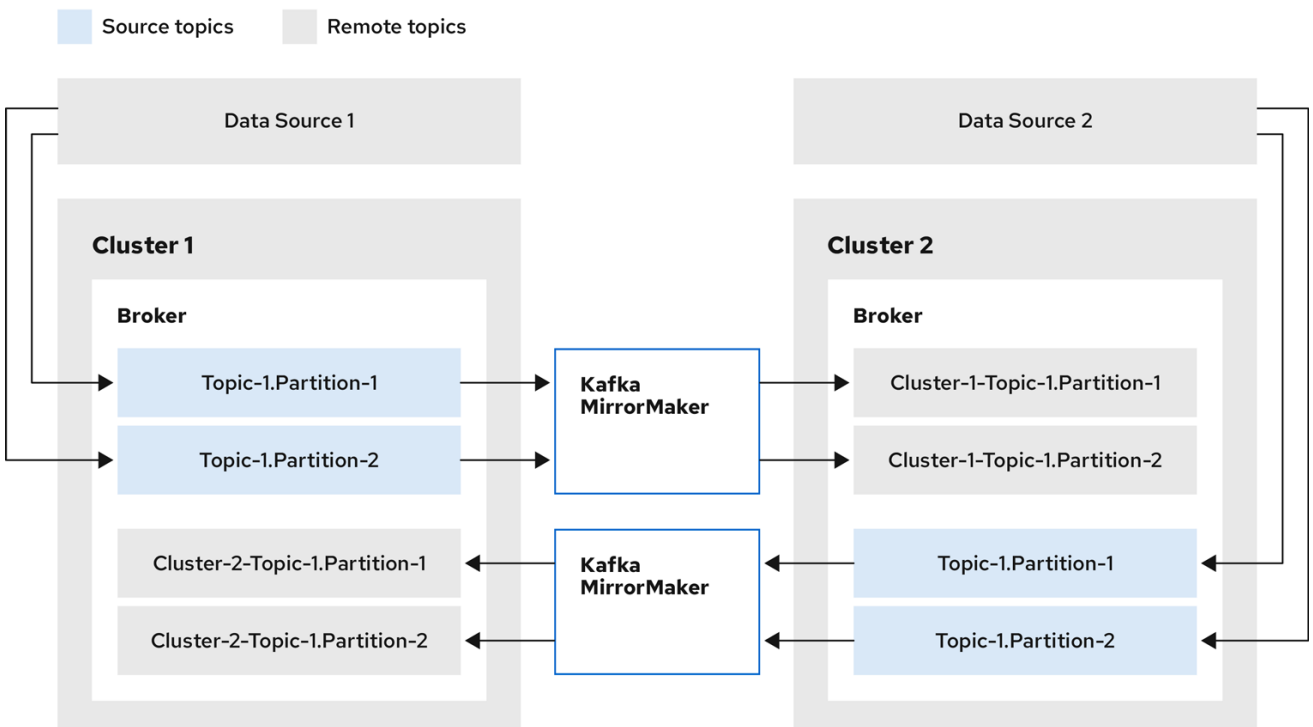
Figure 7.2. Bidirectional replication
