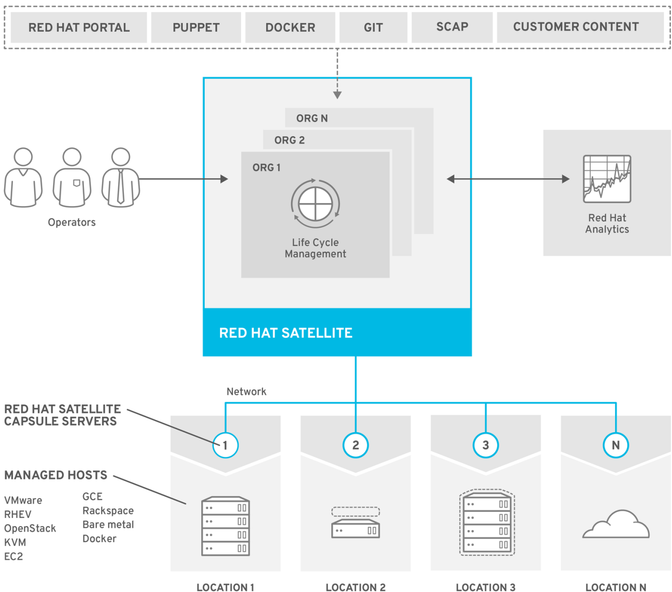
Figure 1.1. Red Hat Satellite 6 System Architecture
