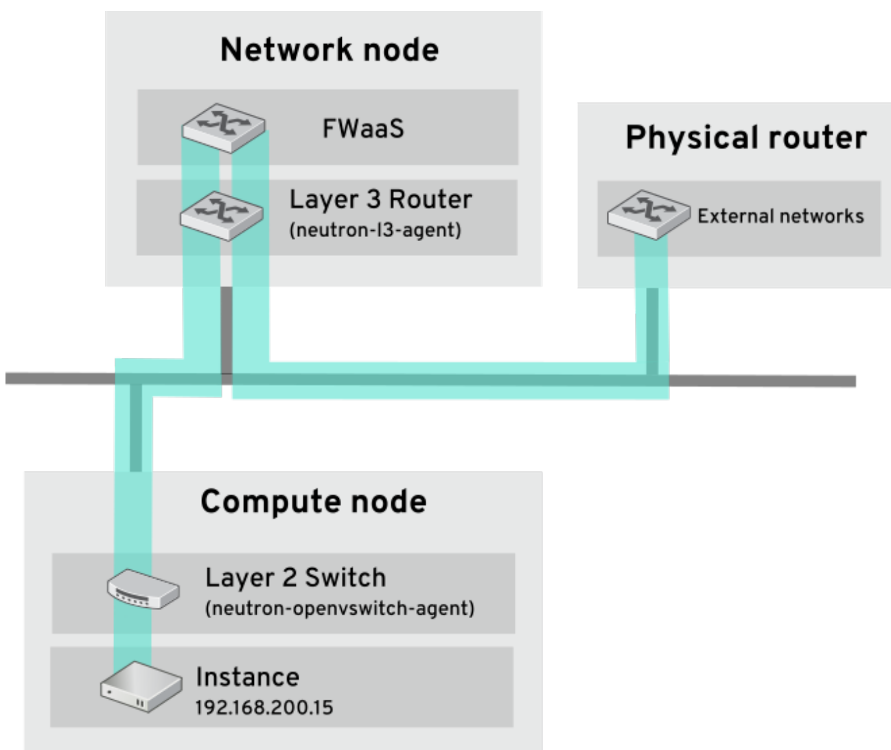
Figure 1. FWaaS architecture
