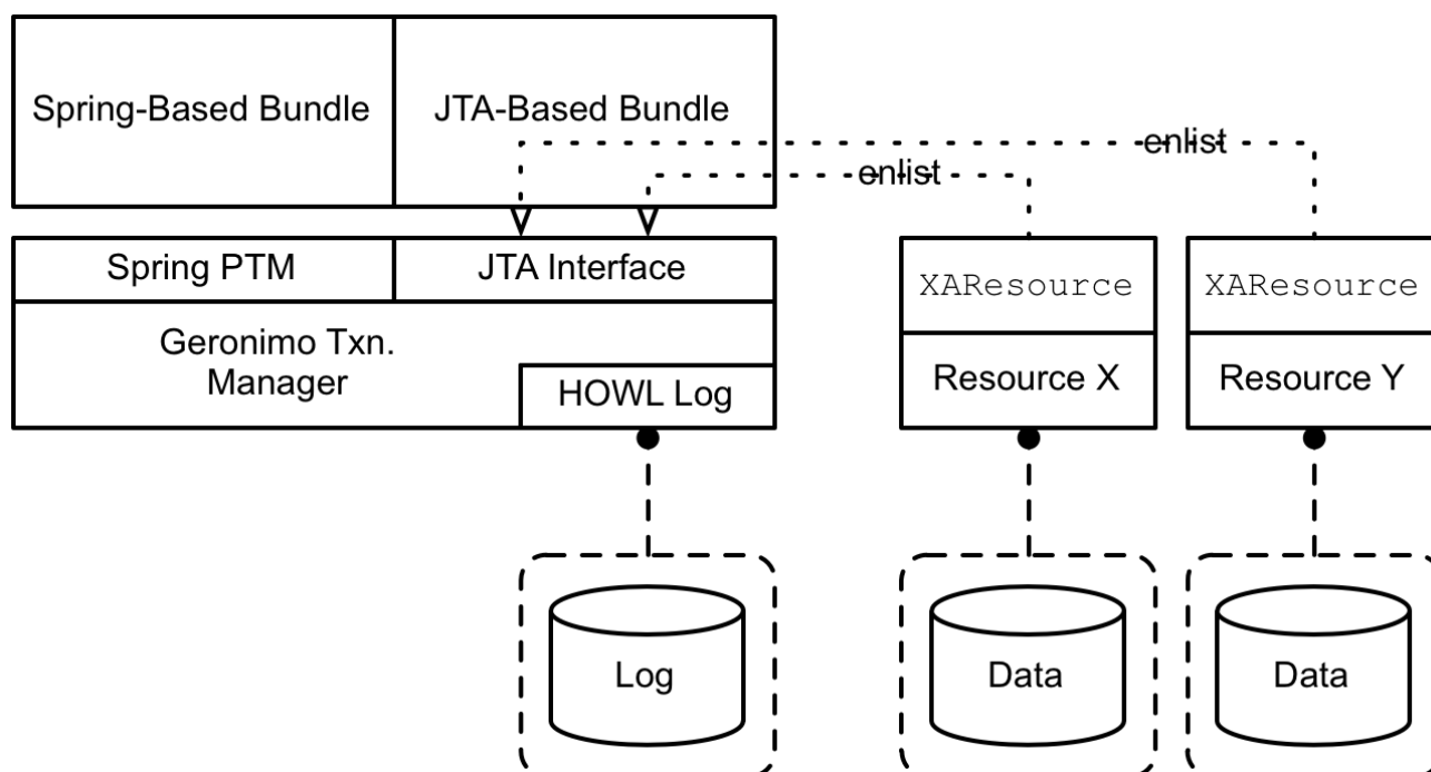
Figure 6.1. OSGi Transaction Architecture
