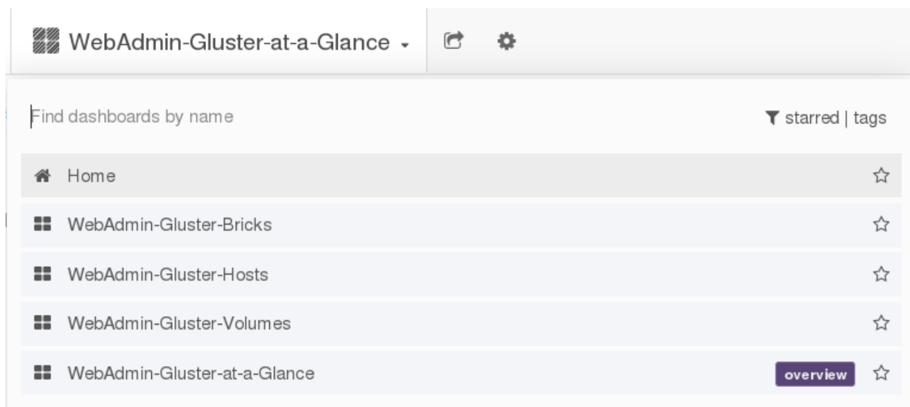
Figure 8.2. Dashboard Selector
