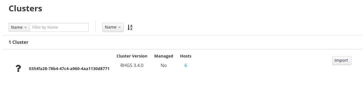
Figure 2.2. Import Cluster
