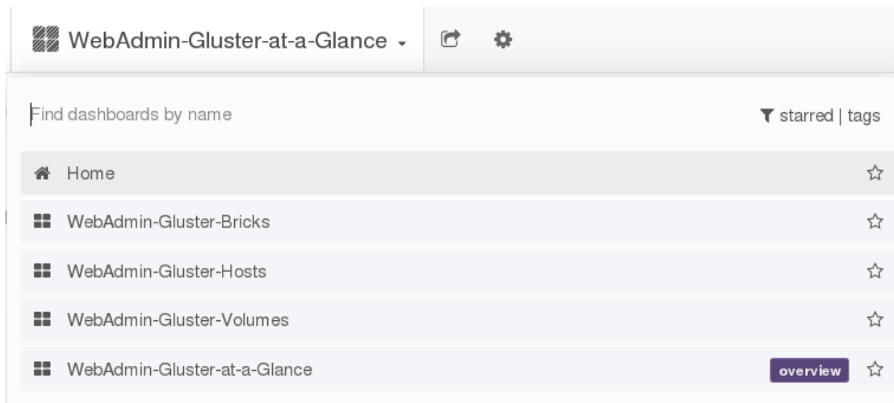
Figure 7.1. Dashboard Selector
