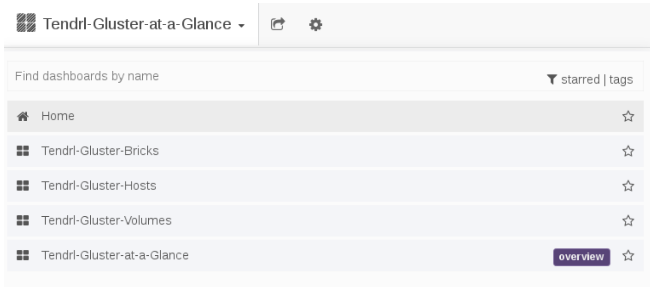
Figure 8.1. Dashboard Search
