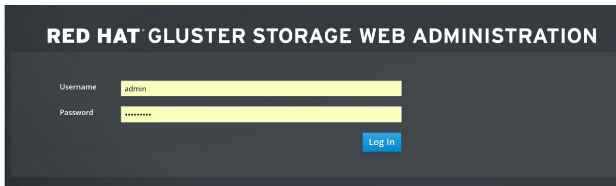
Figure 2.1. Login Page
