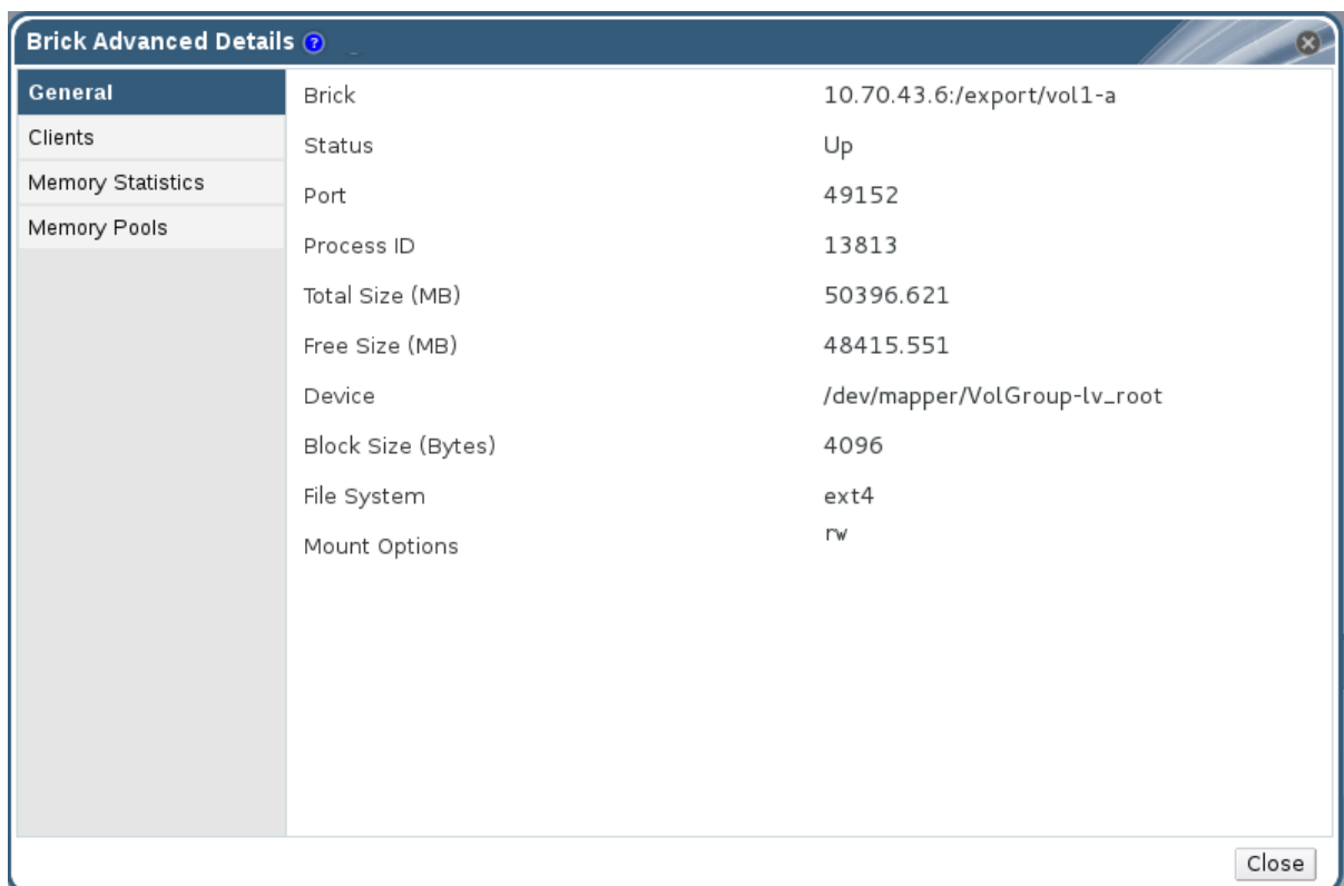
Figure 7.6. Brick Advanced Details
