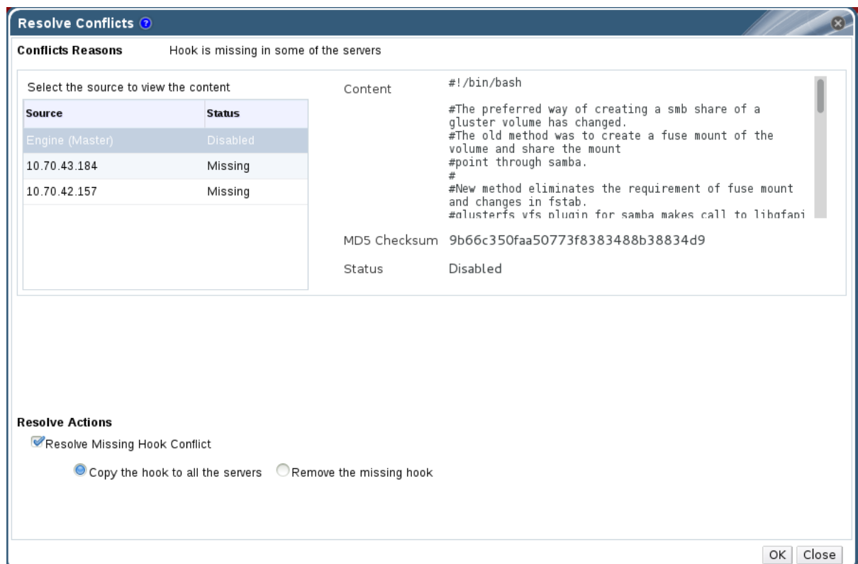
Figure 8.3. Missing Hook Conflict
