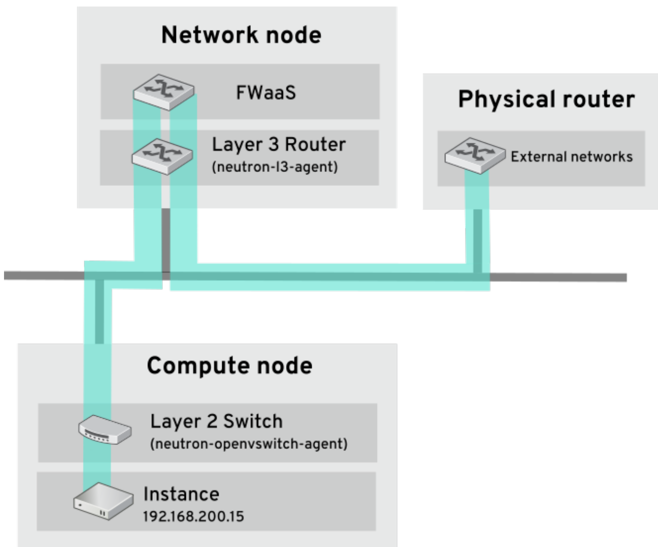
Figure 1. FWaaS architecture
