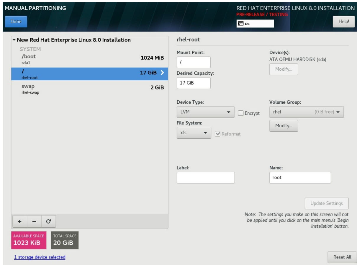
Figure 10.2. Customizing Partitions
