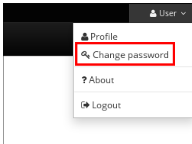
Figure 5.1. Resetting Password
