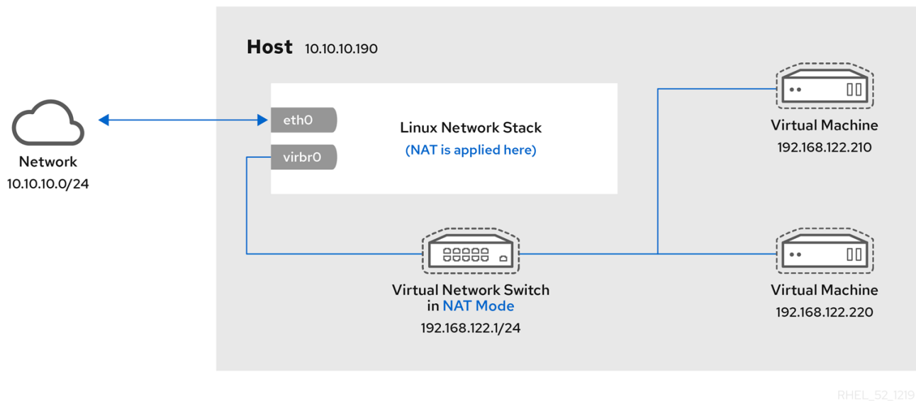
Figure 17.3. Virtual network switch using NAT with two guests
