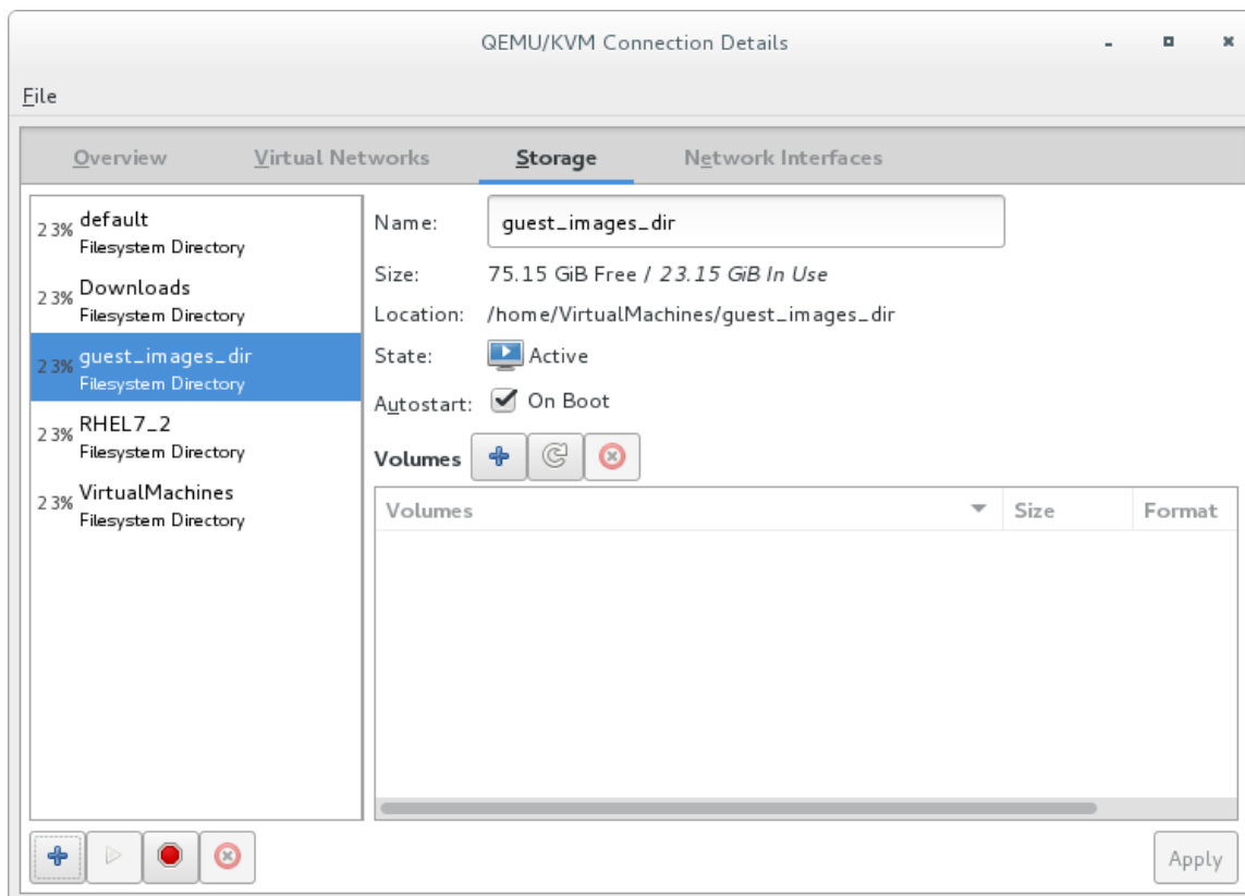
Figure 13.13. Storage tab
