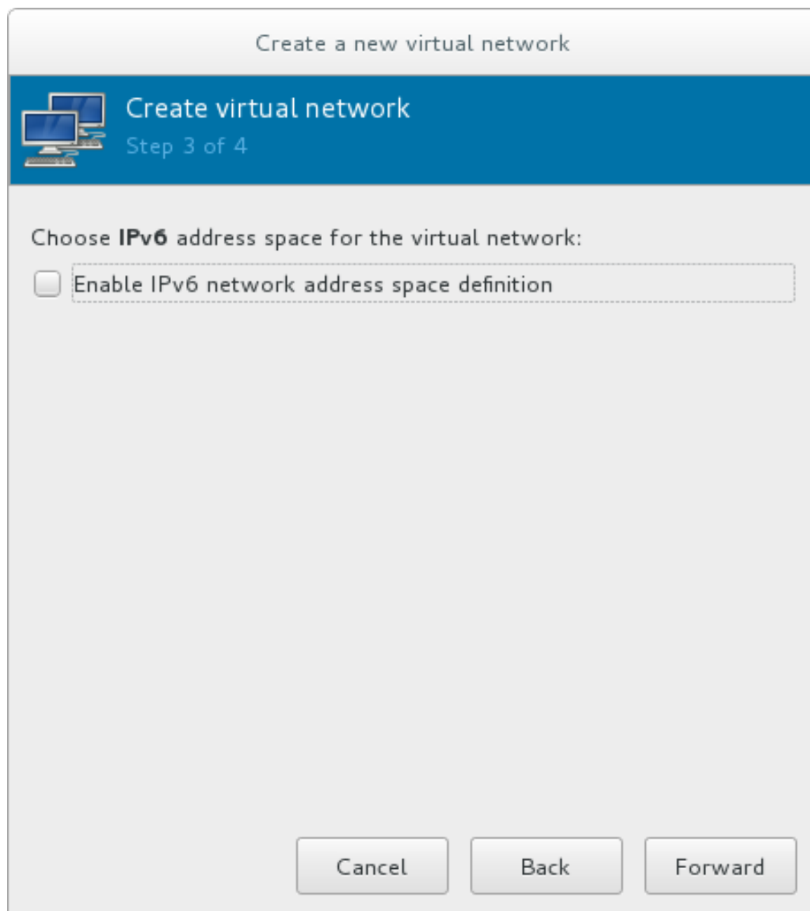
Figure 17.15. Enabling IPv6
