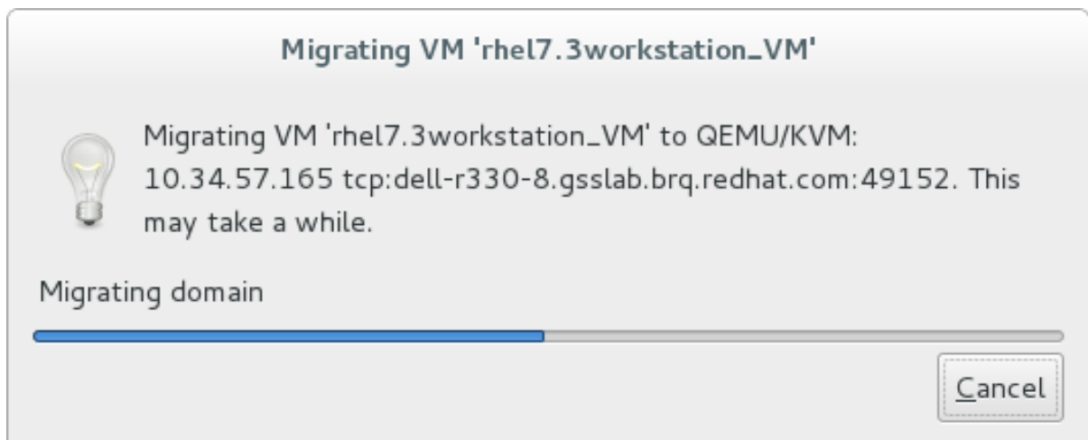
Figure 15.4. Progress window
