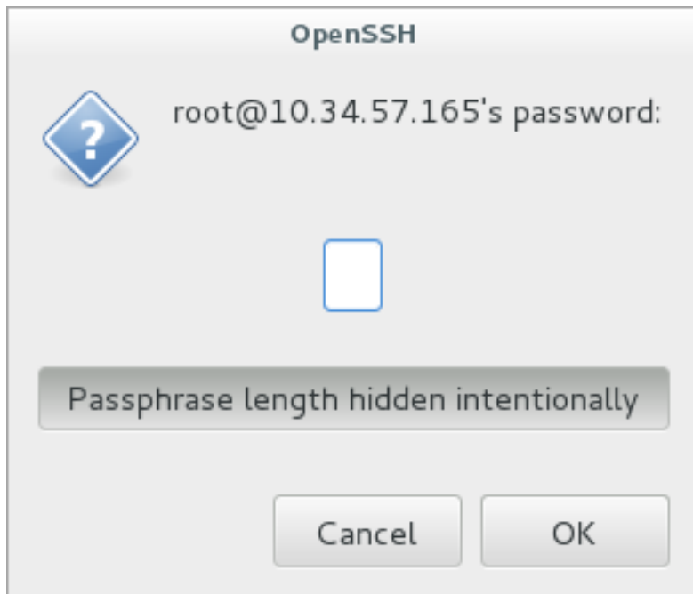
Figure 15.2. Enter password
