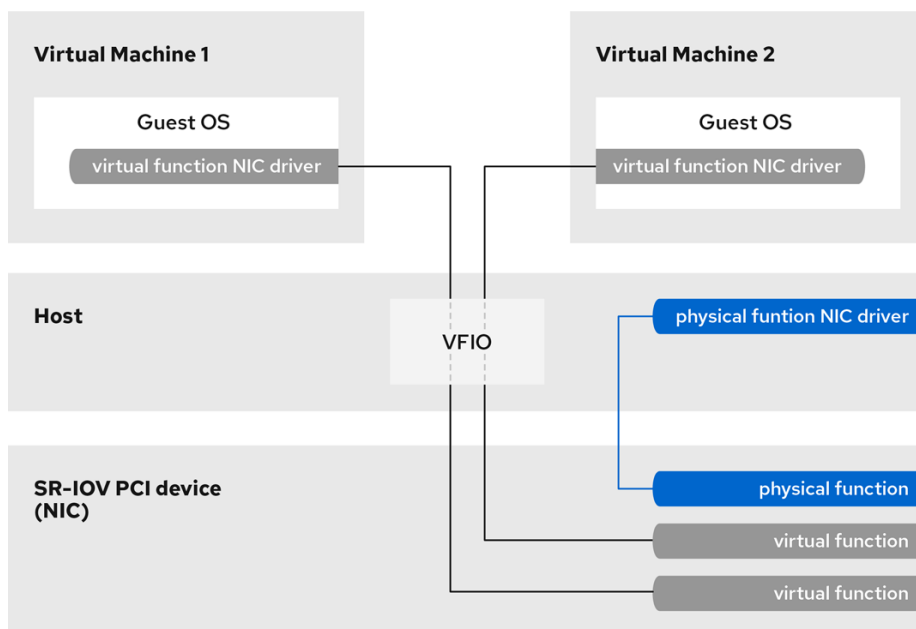
Figure 16.10. How SR-IOV works
