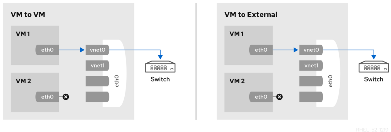
Figure 17.26. Passthrough mode
