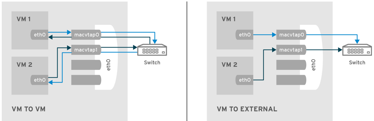
Figure 17.23. VEPA mode
