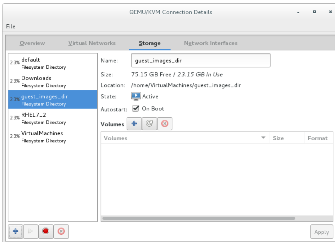
Figure 13.11. Storage tab
