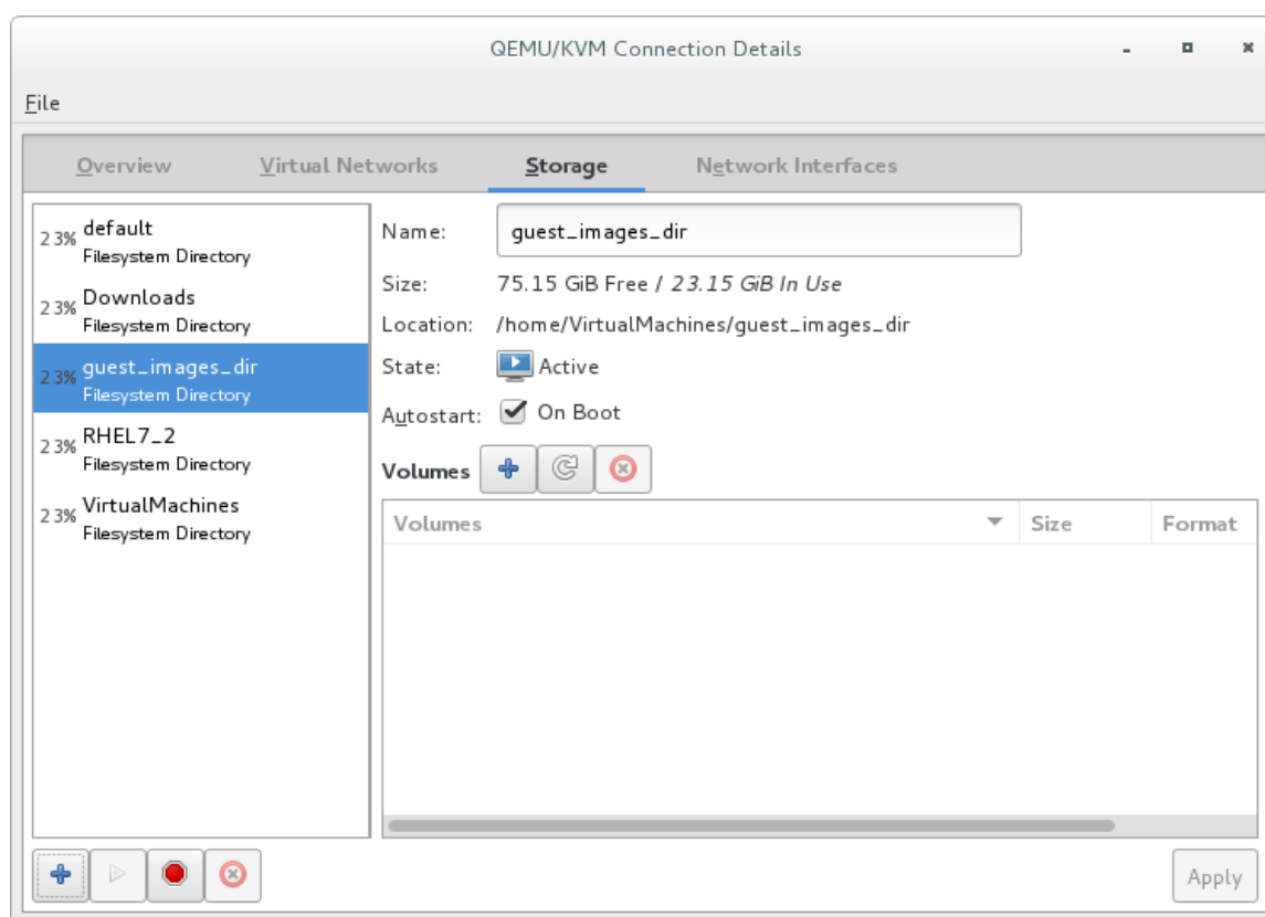
Figure 13.1. Storage tab
