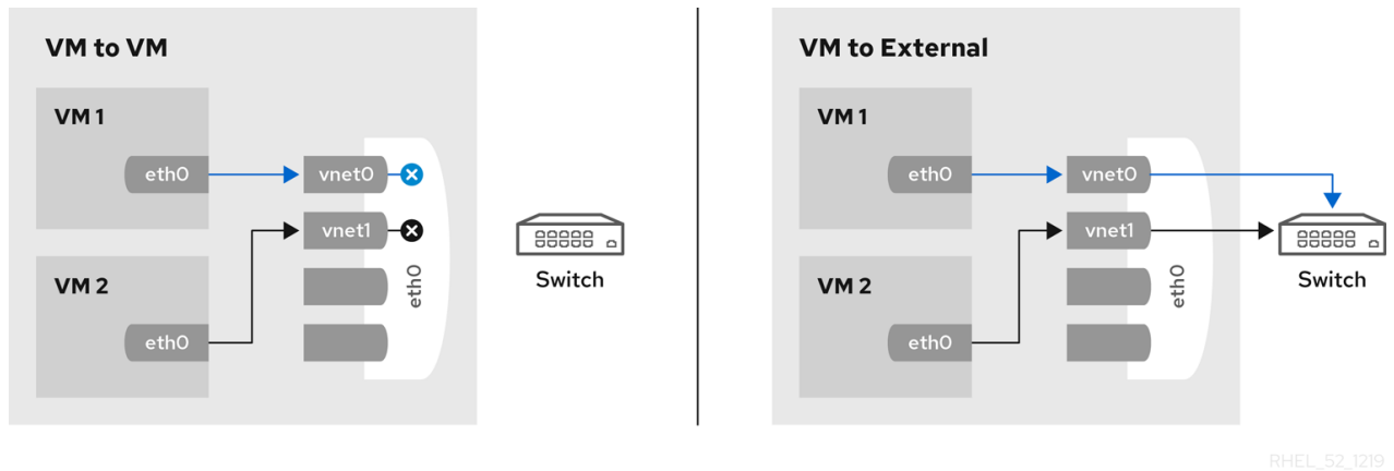
Figure 17.25. Private mode
