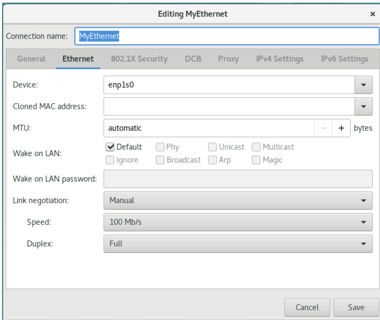
Figure 5.1. Configure 802.3 link settings using nm-connection-editor
