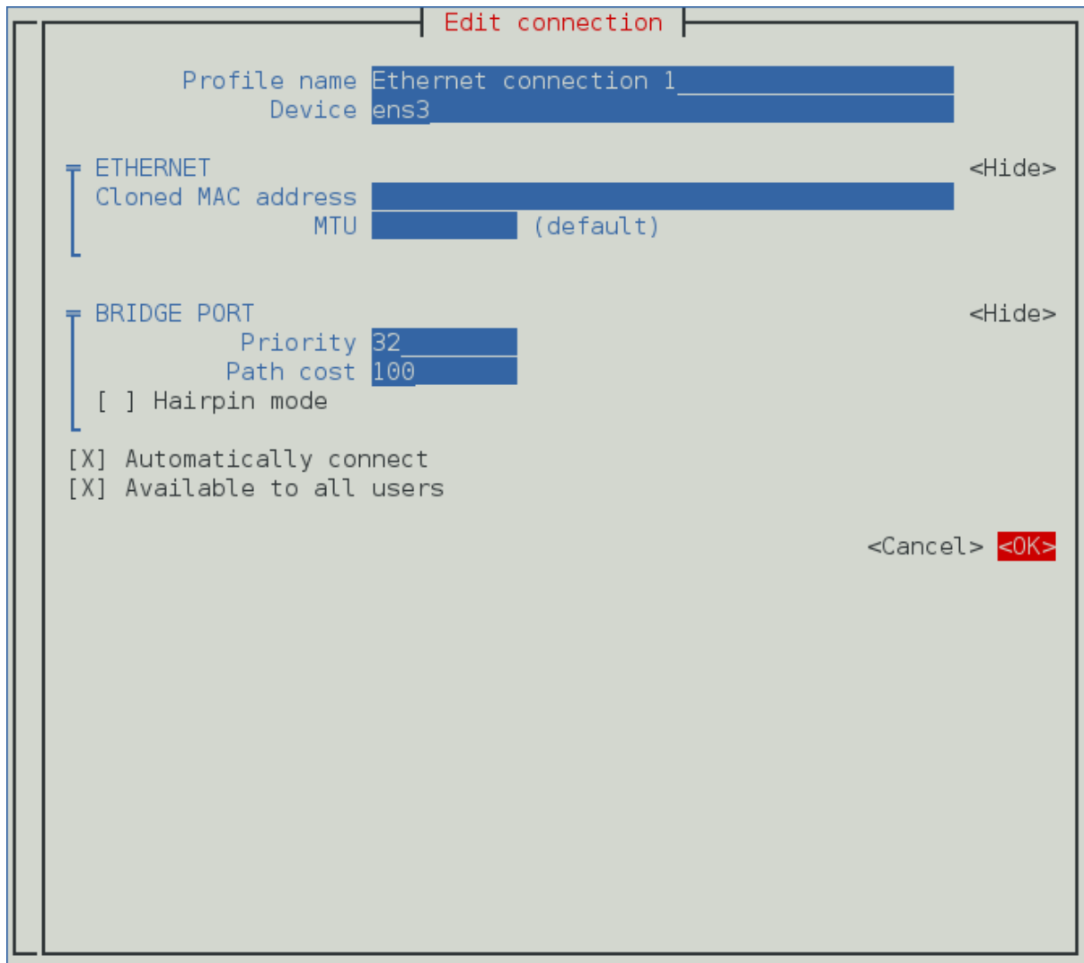
Figure 9.3. The NetworkManager Text User Interface Configuring a BridgeSlave Connection menu
