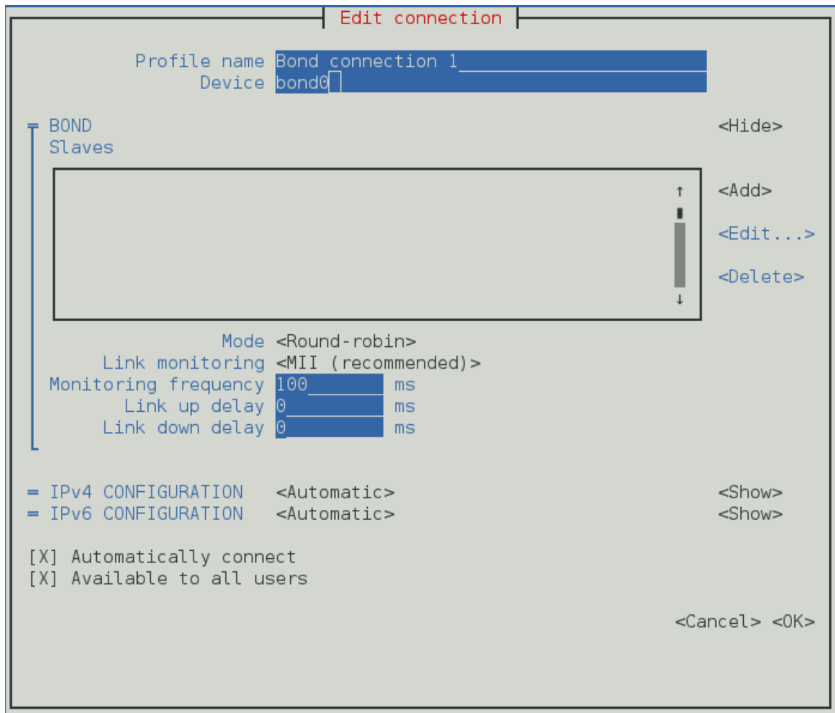
Figure 7.2. The NetworkManager Text User Interface Configuring a Bond Connection menu
