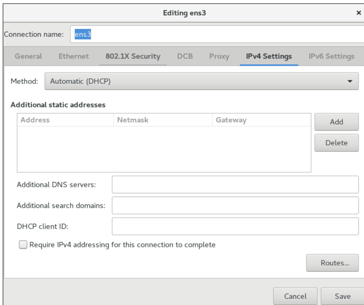
Figure 5.3. Configuring IPv4 Settings
