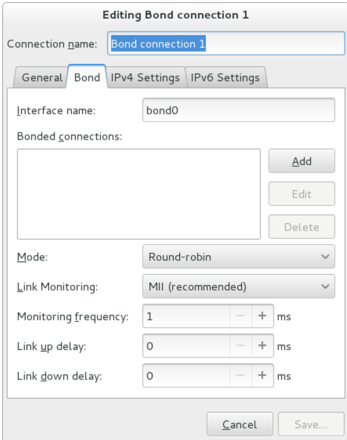
Figure 7.6. The NetworkManager Graphical User Interface Add a Bond menu
