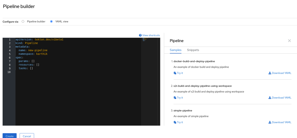
Figure 4.1. YAML view
