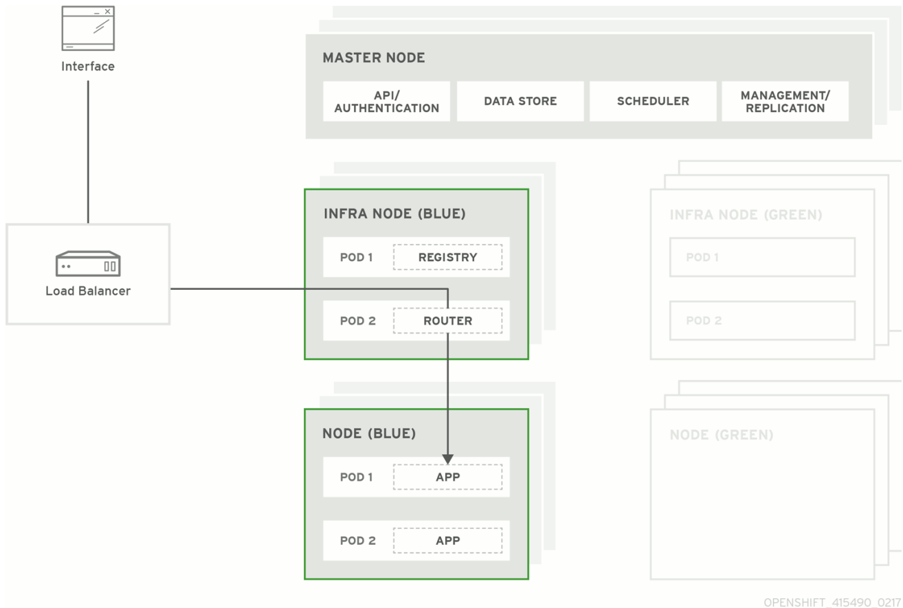
Figure 5.1. Blue-Green Deployment
