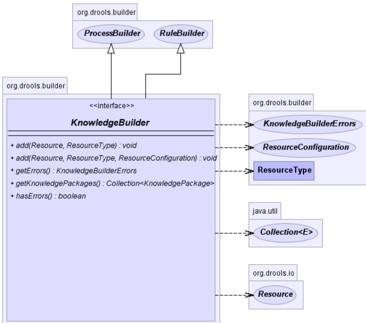
Figure 5.3. KnowledgeBuilder Chart
