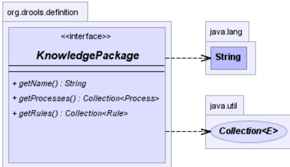
Figure 6.1. KnowledgePackage interface
