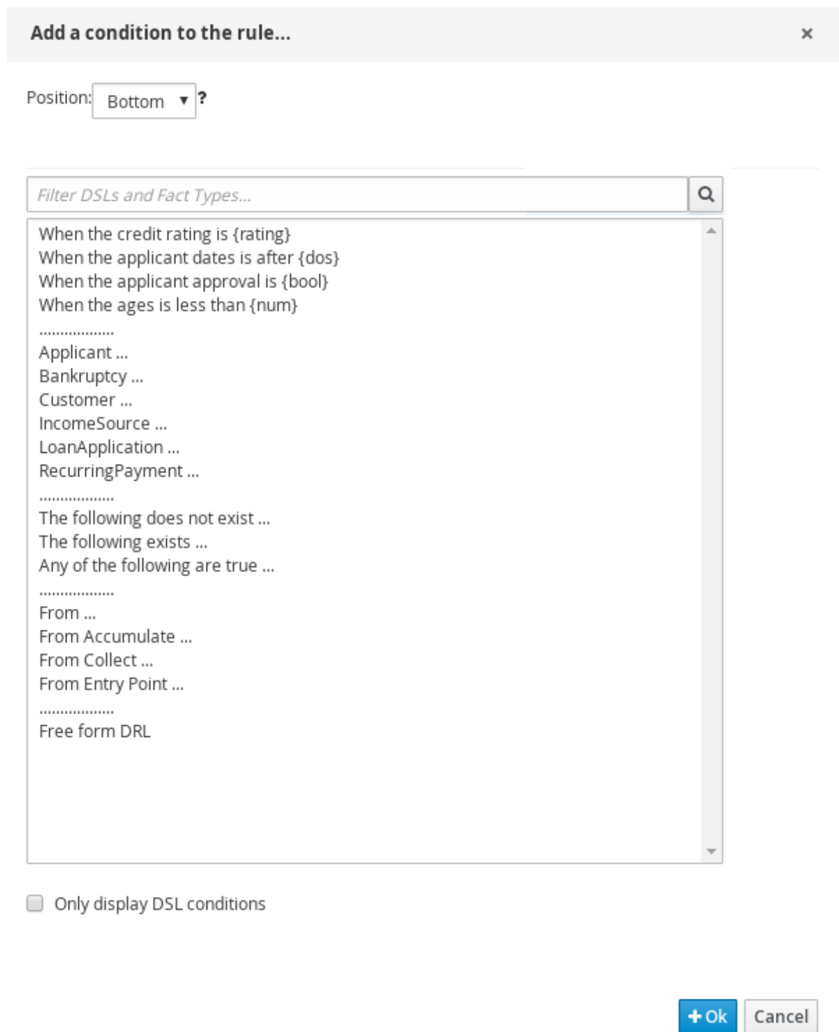
Figure 58.2. Add a condition to the rule
