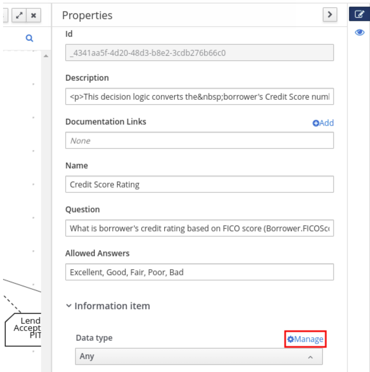
Figure 6.26. Managing data types in decision requirements diagram (DRD) properties
