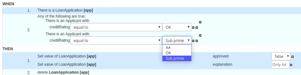
Figure 35.2. Example enumeration drop-down options in a guided rule or guided rule template
