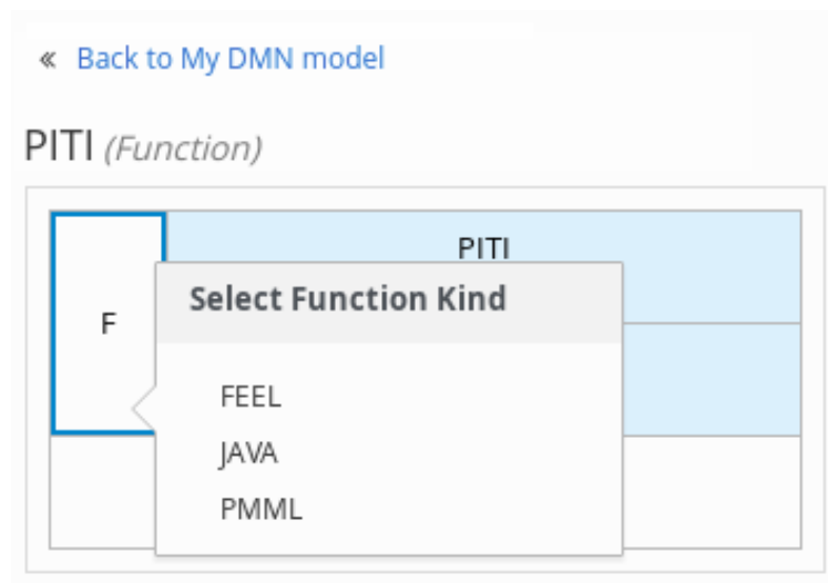
Figure 6.5. Selecting the function or other logic type for a business knowledge model
