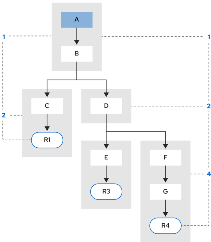
Figure 83.4. Example 3: Three rules with pattern sharing
