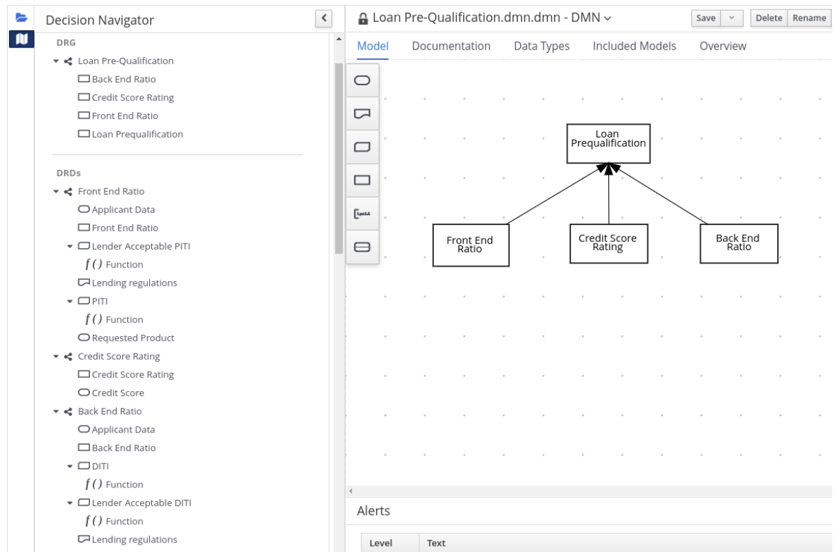
Figure 6.52. Multiple nested DRDs for loan prequalification
