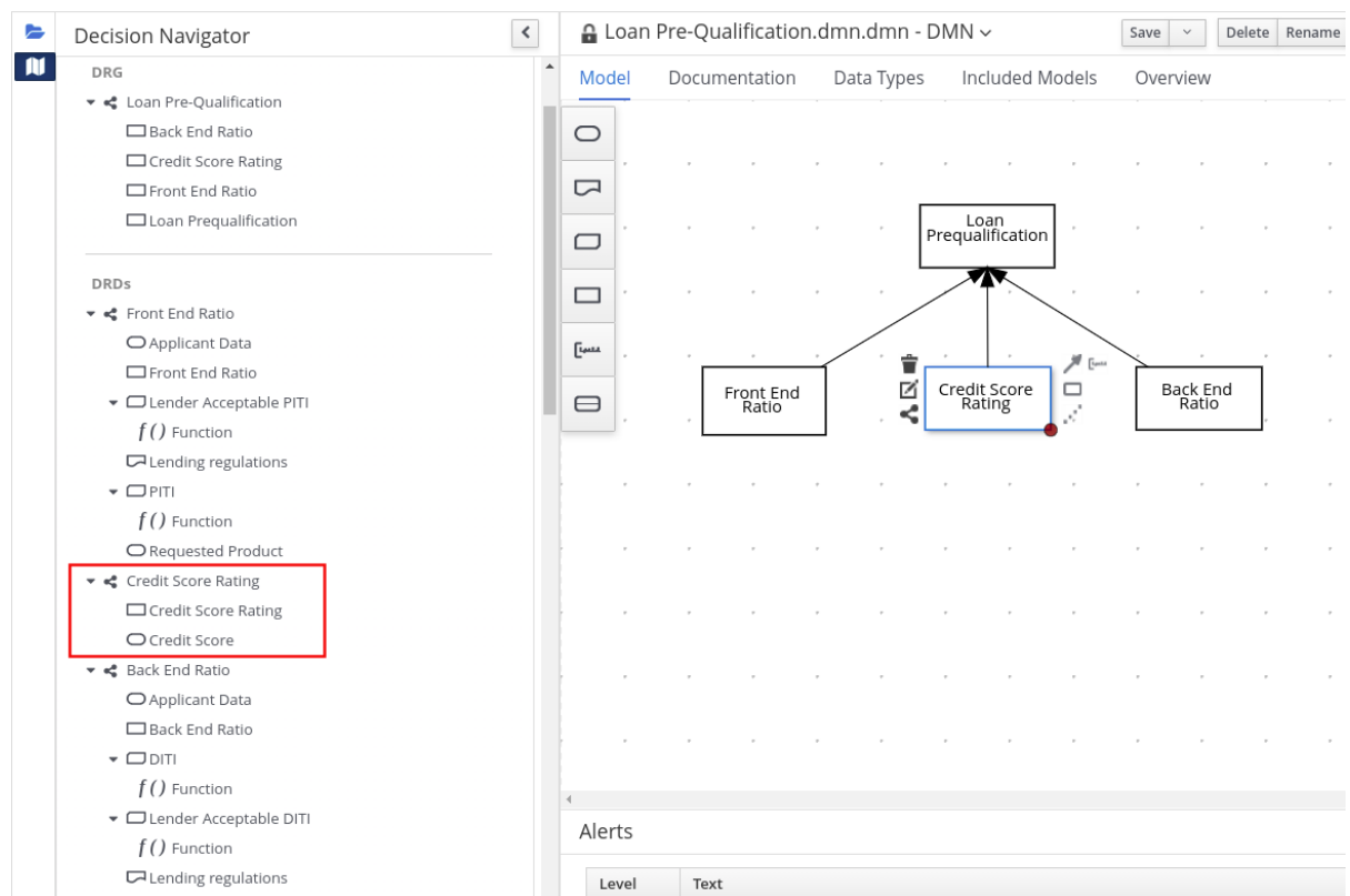
Figure 6.55. Overview of credit score rating DRD
