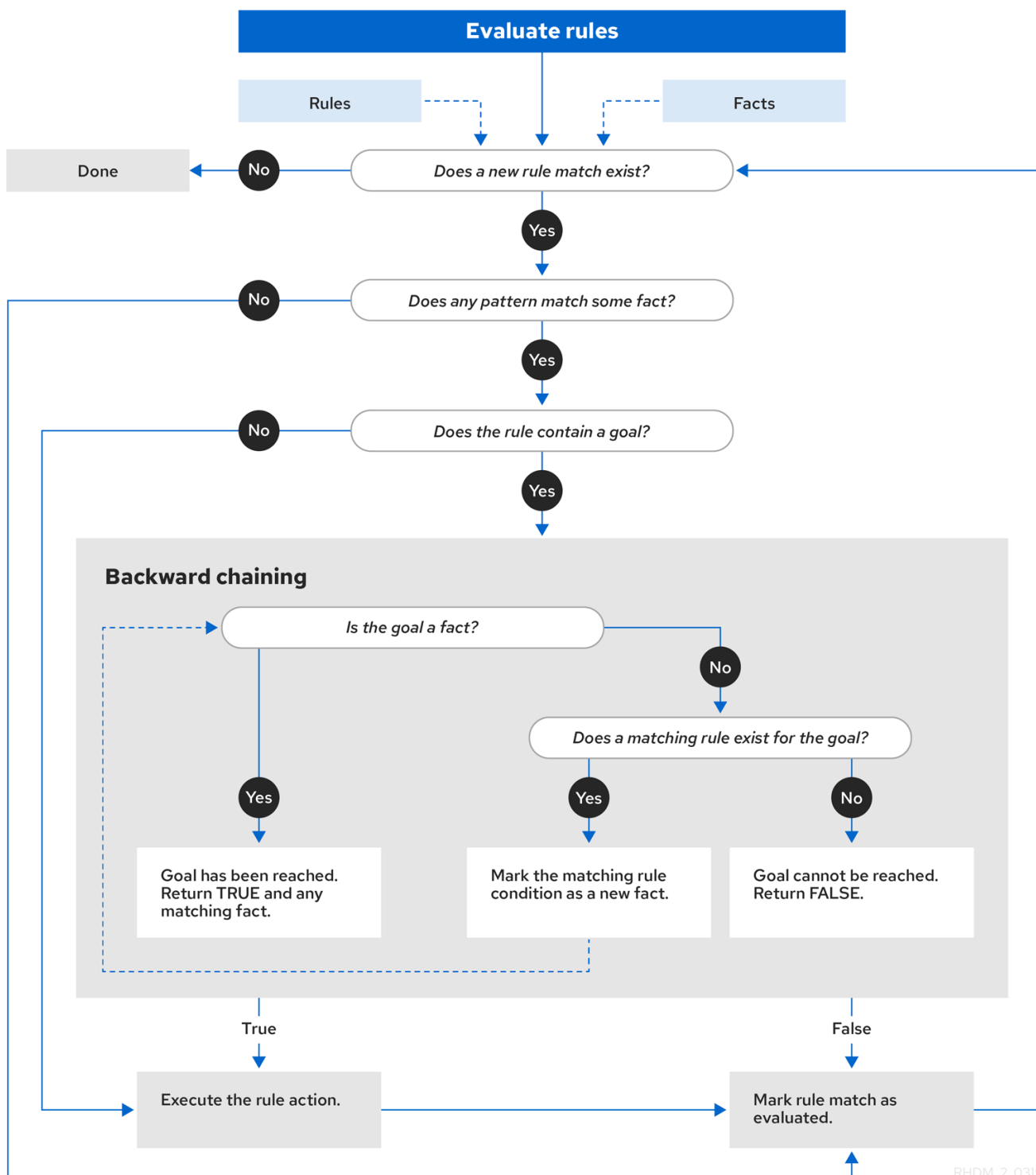
Figure 87.4. Rule evaluation logic using forward and backward chaining
