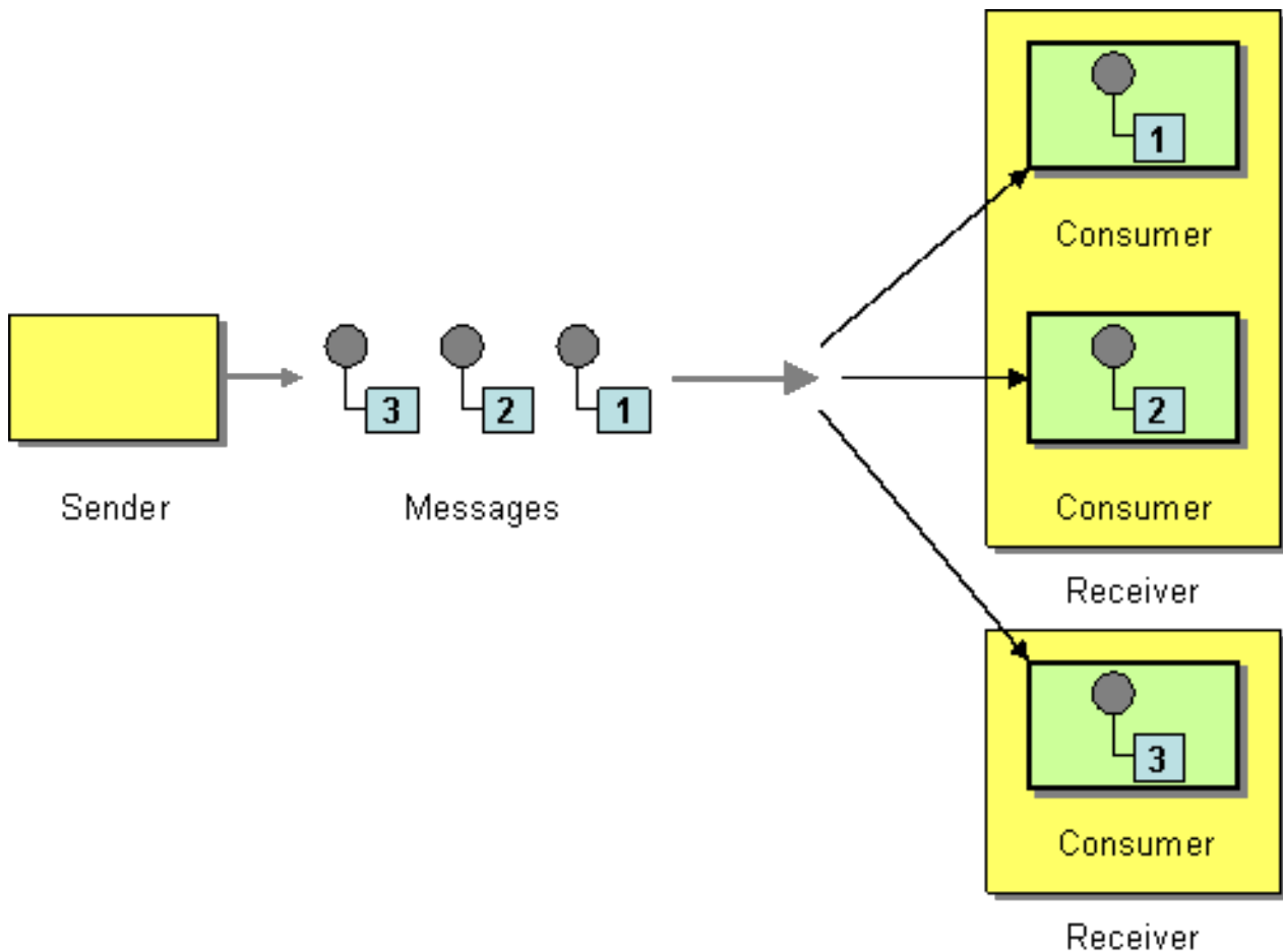
Figure 10.3. Competing Consumers Pattern
