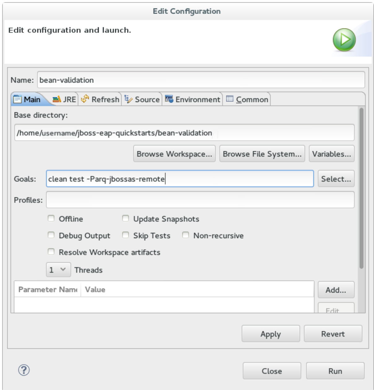
Figure 5.6. Edit Configuration
