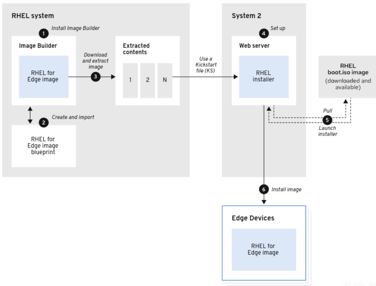
Figure 1.2. Deploying RHEL for Edge in network-based environment
