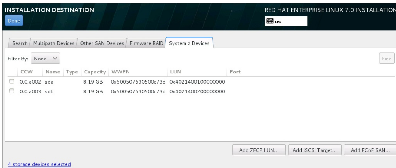
Figure 18.26. Tabbed Overview of Specialized Storage Devices
