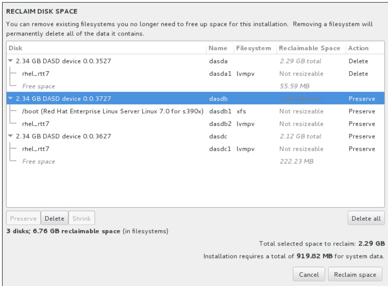
Figure 18.17. Reclaim Disk Space from Existing File Systems
