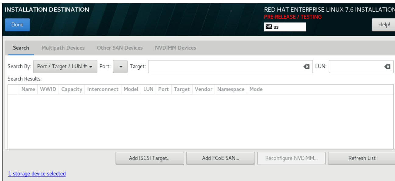
Figure 13.30. The Storage Devices Search Tab
