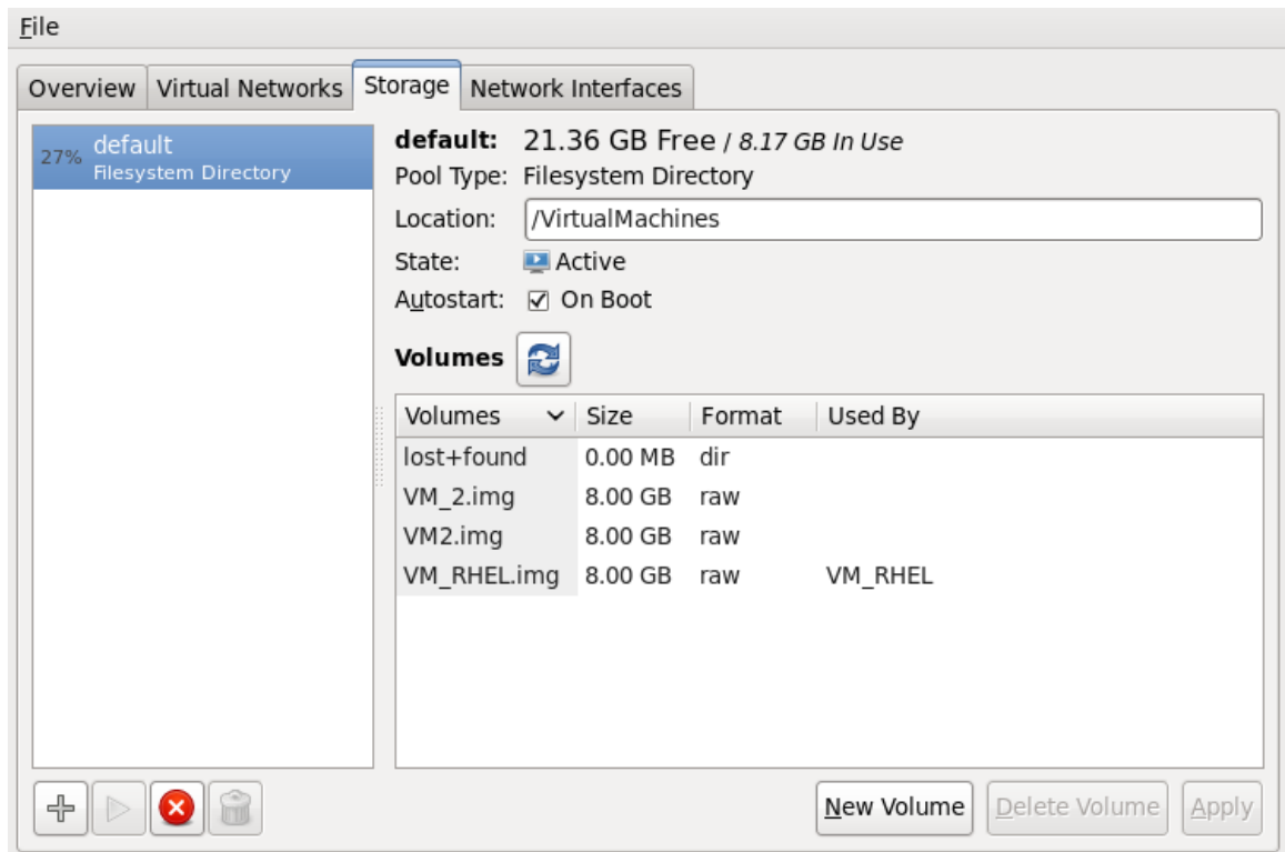
Figure 12.13. Storage tab
