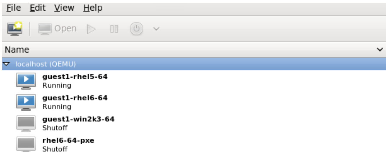
Figure 15.1. Starting virt-manager
