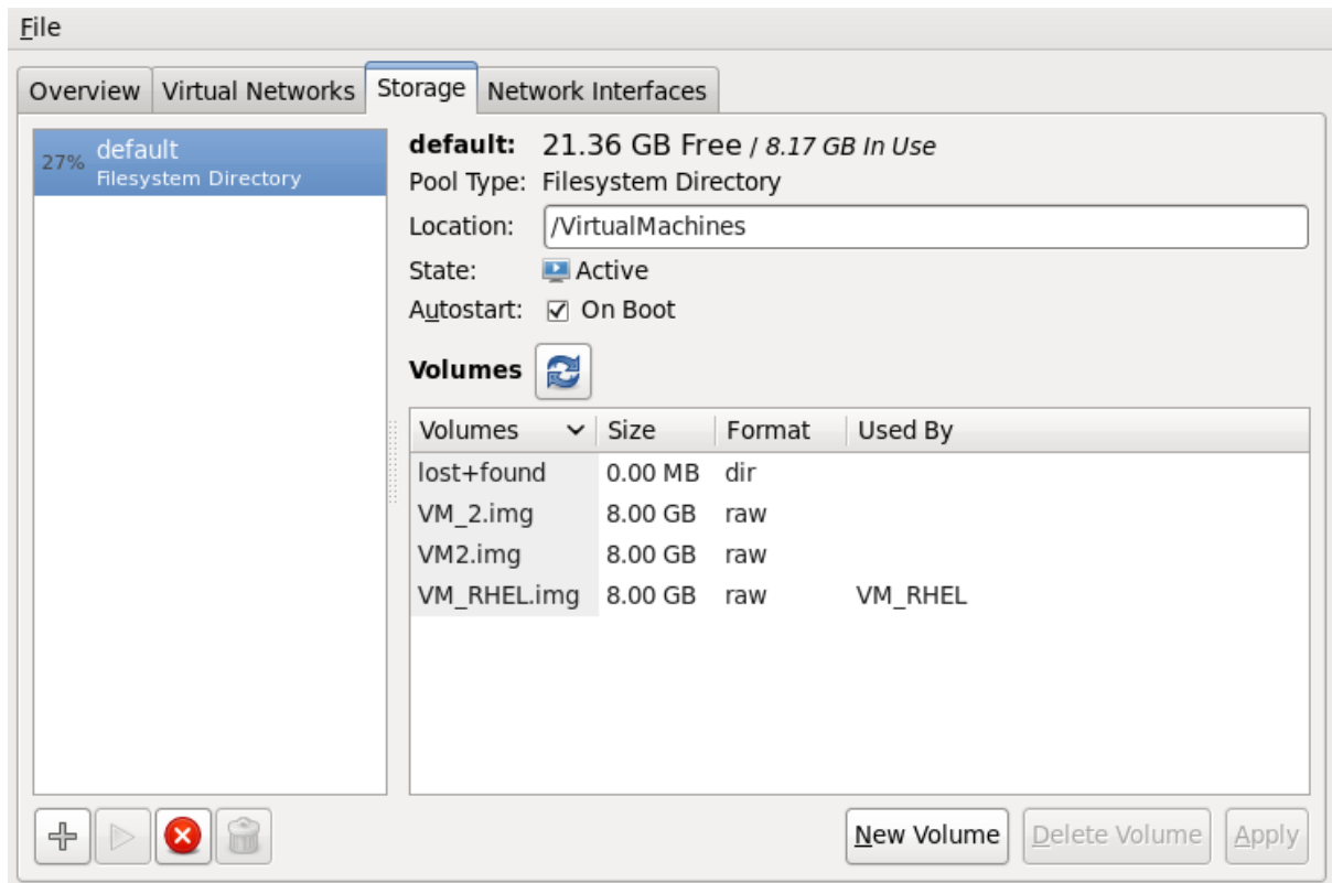
Figure 12.23. Stop Icon
