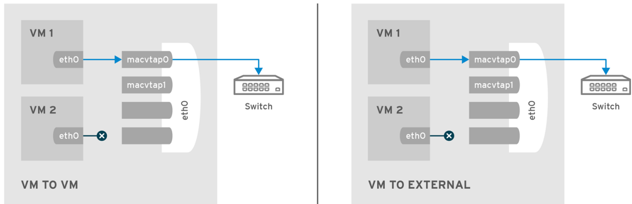
Figure 18.26. Private mode
