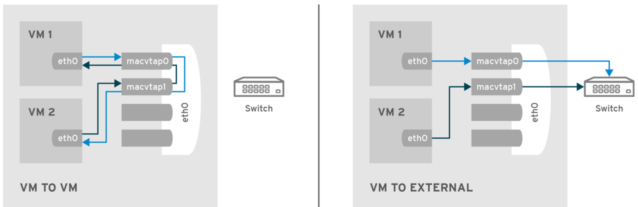
Figure 18.25. Bridge mode
